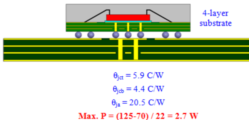
Figure 15. 324 ball, 19mm x 19mm BGA with 4-Layer Substrate
