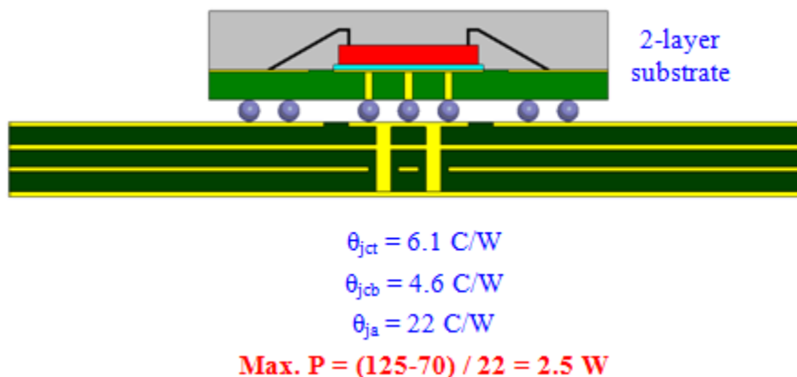
Figure 14. 324 ball, 19mm x 19mm BGA with 2-Layer Substrate
