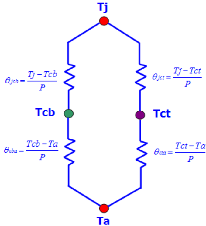
Figure 9. Redefined \theta_{ja} and Partial Resistances
