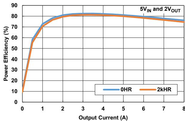
Figure 4. Number 4 Pre and Post High Power Test Efficiency Curves
