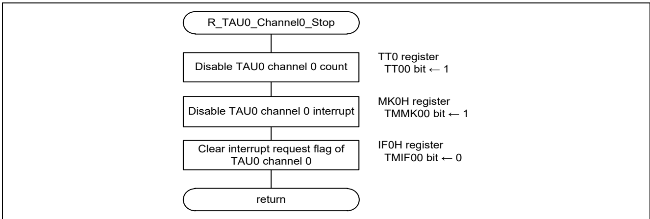
Figure 6.29 Disabling TAU00
