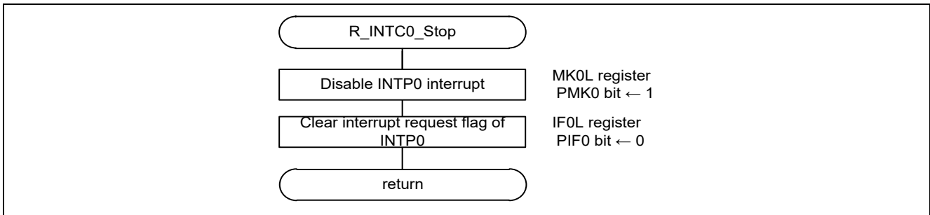
Figure 6.28 Disabling INTP0
