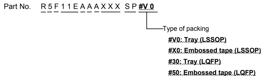
Figure 1 - 1 Part Number, Memory Size, and Package of RL78/G1G
