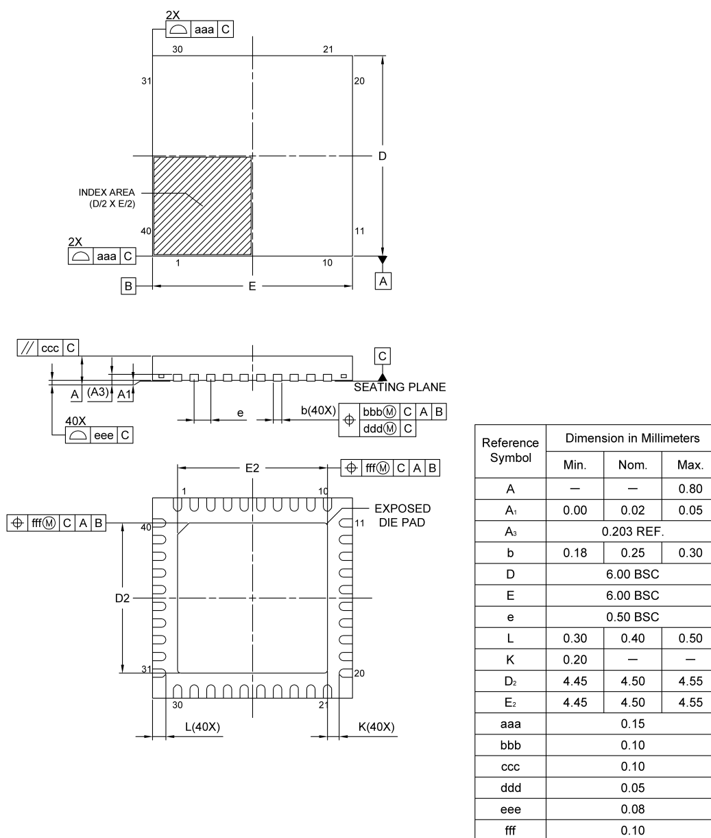
Figure 1. 40-pin HWQFN (PWQN0040KD-A)
