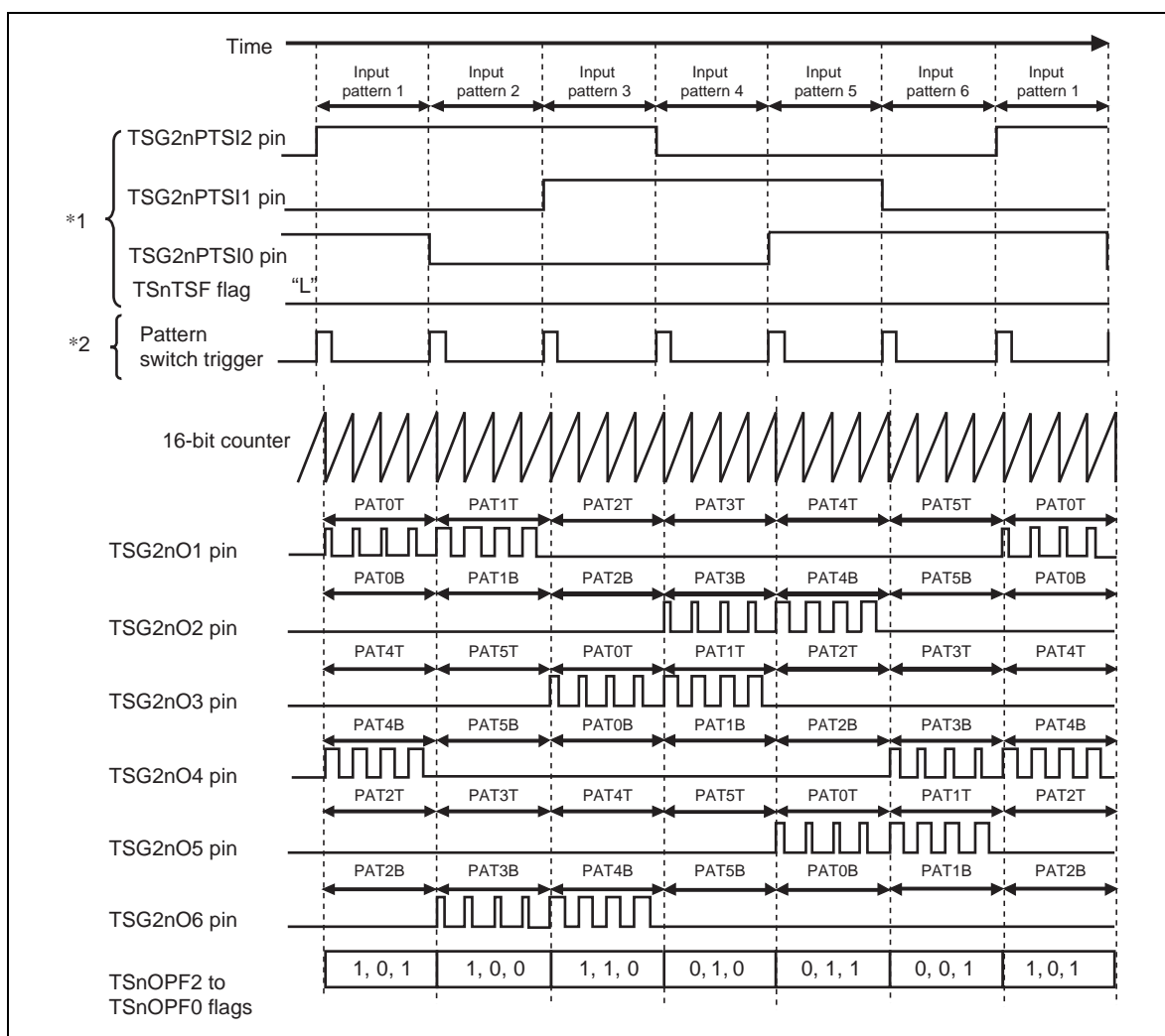
Figure 15-65 Example of Operation in 120-DC Mode (Normal Rotation: TSnSTR1.TSnTSMF = 0 and TSnOPT0.TSnIDC = 0)
