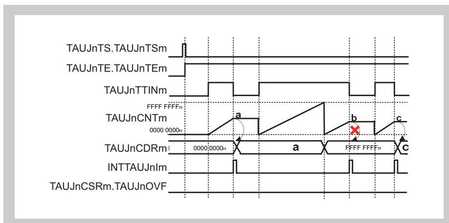
Figure 14-31 TAUJnCMORM.TAUJnCOS[1:0] = 10 B , TAUJnCMORM.TAUJnMD0 = 0, TAUJnCMURm.TAUJnTIS[1:0] = 11 B
