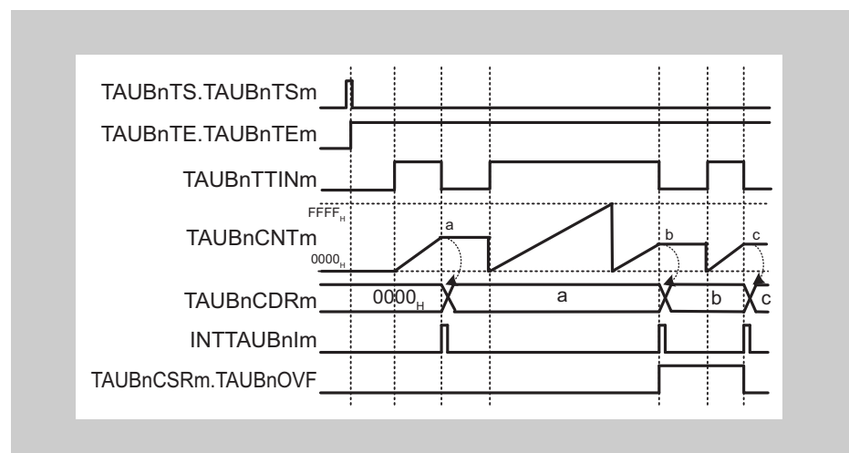
Figure 13-35 General Timing Diagram of TAUBnTTINm Input Signal Width Measurement Function
