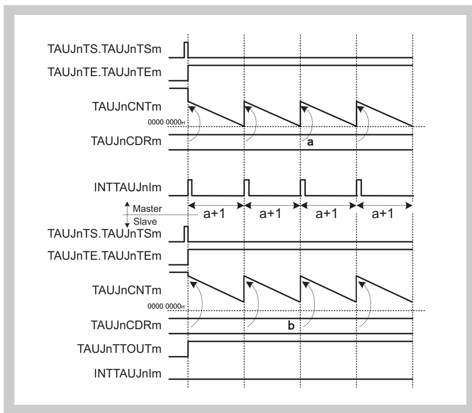
Figure 14-42 TAUJnCDRm (Slave) \geq TAUJnCDRm (Master) + 1, Positive Logic (TAUJnTOL.TAUJnTOLm (Slave) = 0)
