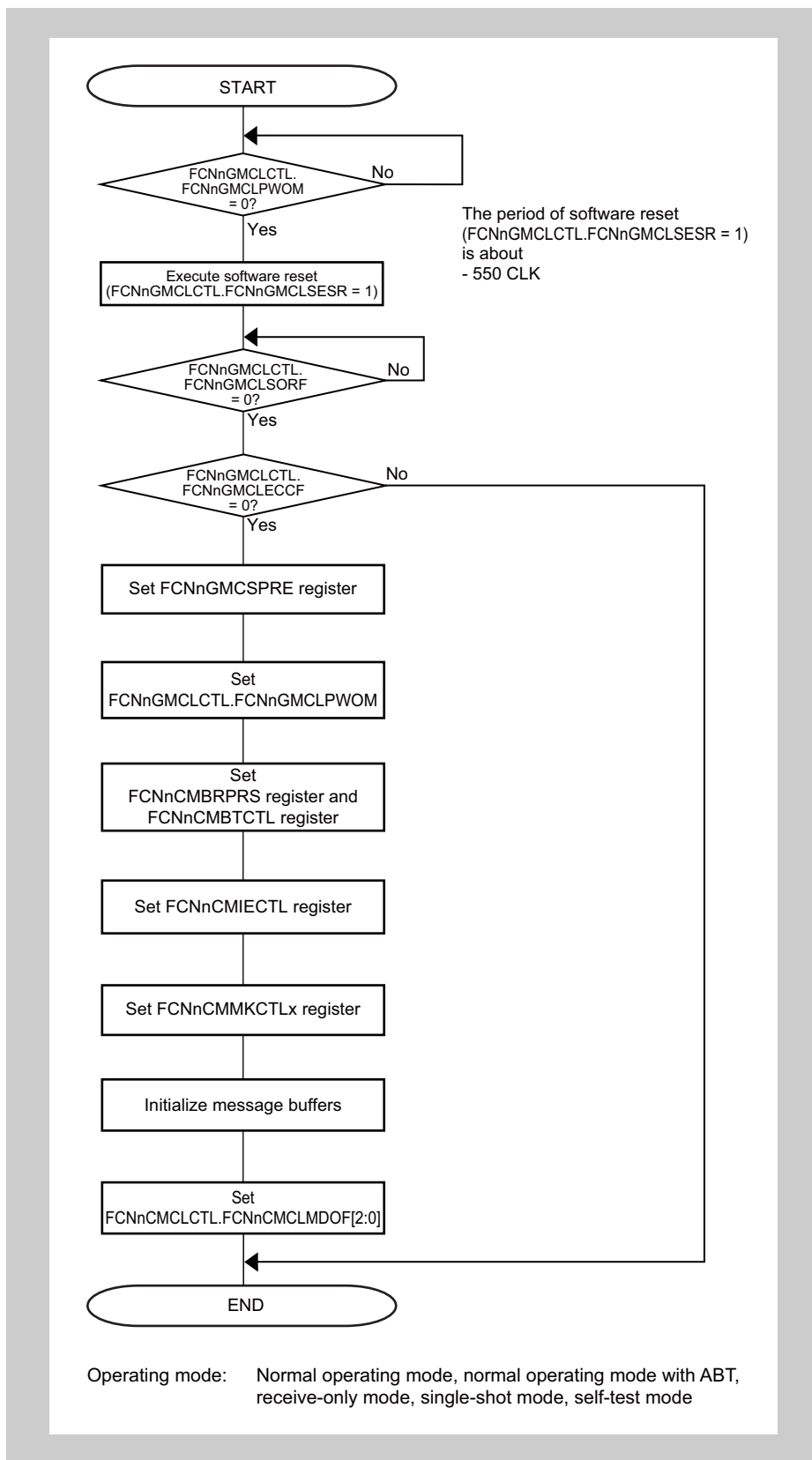
Figure 20-15 Re-initialization with Software Reset Function
