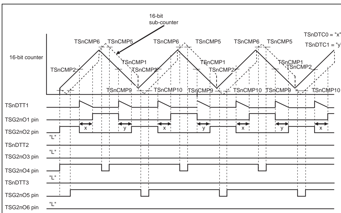
Figure 15-53 Example of Output Waveform with Dead Time in HT-PWM Mode
