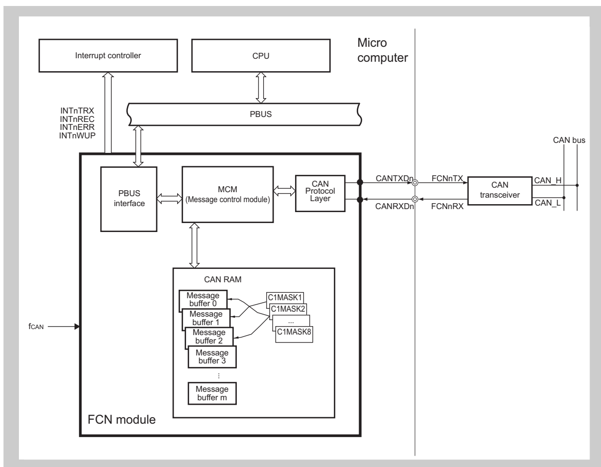
Figure 20-1 Block Diagram of the CAN Controller
