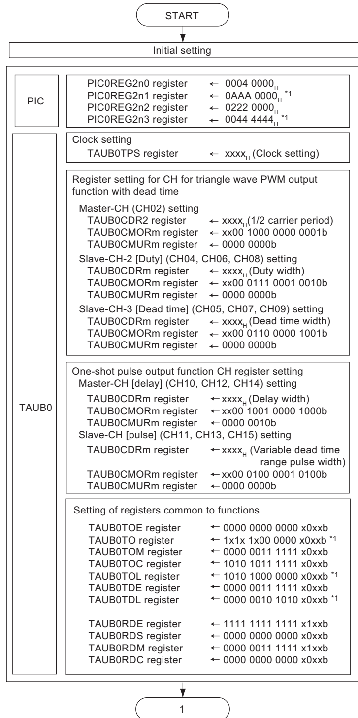
Figure 24-14 Setting Flow (Active High)
