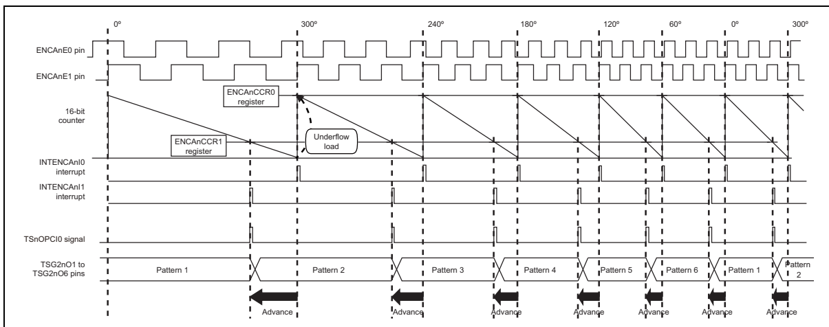
Figure 24-36 Operation Example of Control Method 2: at Down Count
