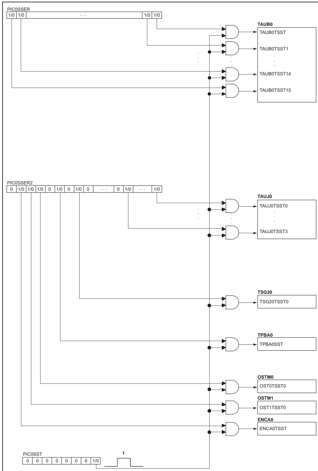
Figure 24-1 Block Diagram
