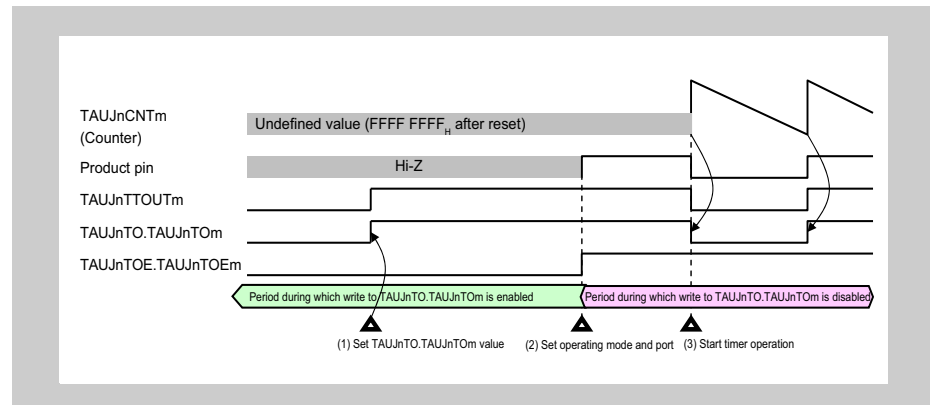
Figure 14-6 General Procedure for Specifying a TAUJnTTOUTm Channel Output Mode
