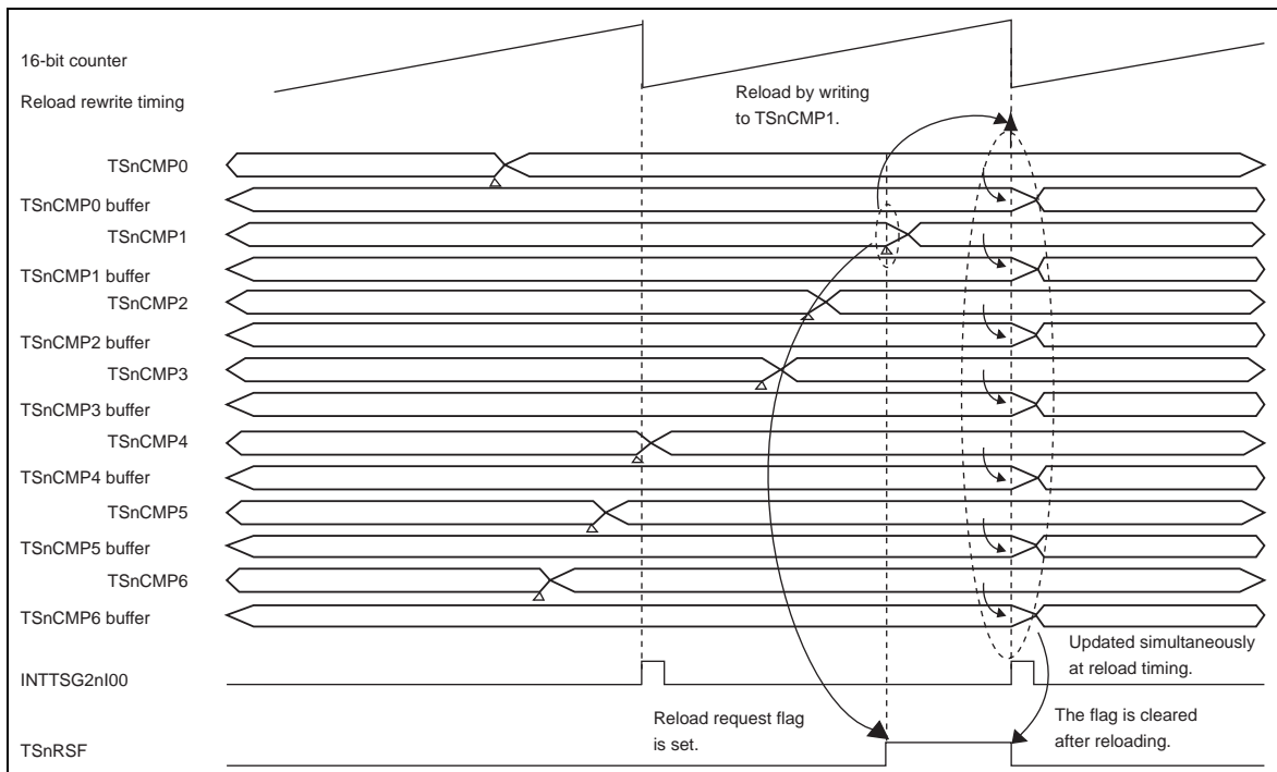
Figure 15-4 Simultaneous Rewrite Timing (2/2) (Example of PWM Mode)
