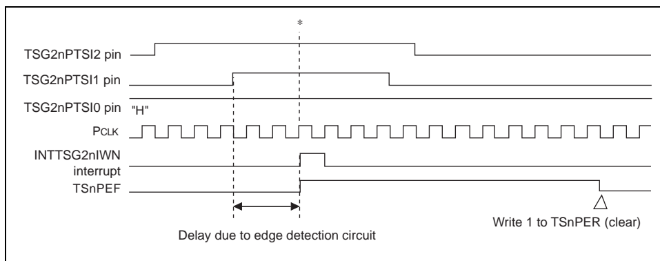
Figure 15-18 Example of Pattern Error Detection Flag Operation (TSG2nPTS12 to TSG2nPTS10 Pins = 111)
