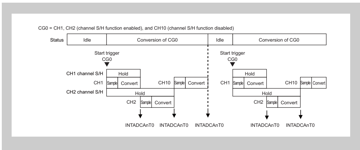
[Example 3: When CG0 is in one-shot conversion mode (no repetition) (ADCA n TRM0 bit = 0)]
