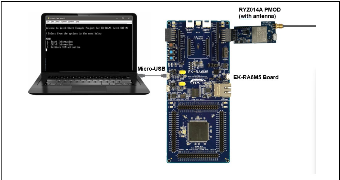
Figure 4. Connecting the EK-RA6M5 Board to the Host PC via USB Full Speed Port
