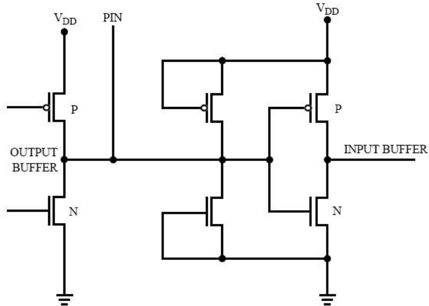
Figure 54. Digital I/O
