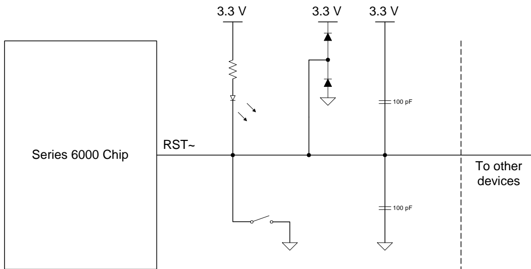
Figure 26. Reset Circuit
