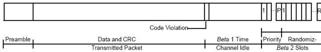
Figure 18. Packet Timing
