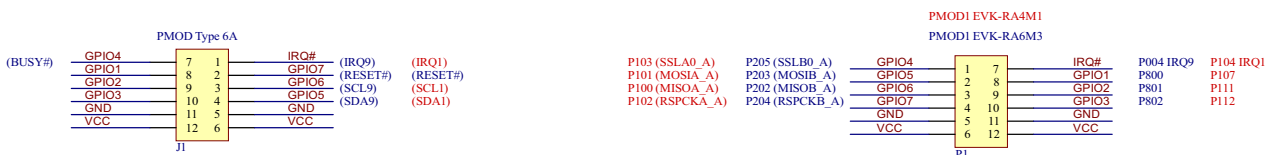
Figure 5. US082-INTERPEVZ Application Schematic
