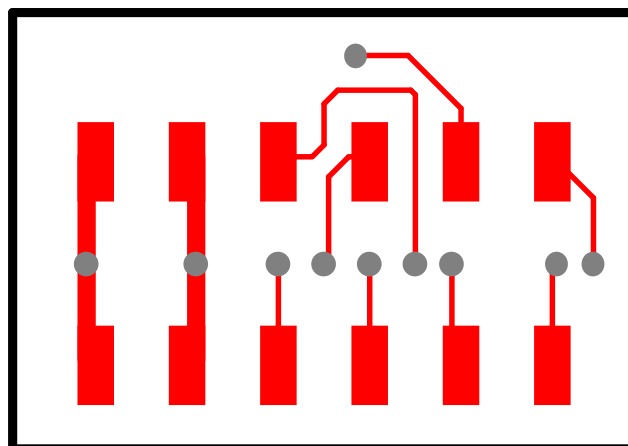
Figure 7. Copper Top
