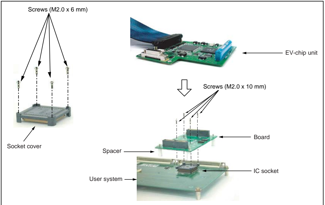
Figure 1 User System Interface Board for the SH7124 PLQP0048JA-A (Former Code: FP-48FV) Package
