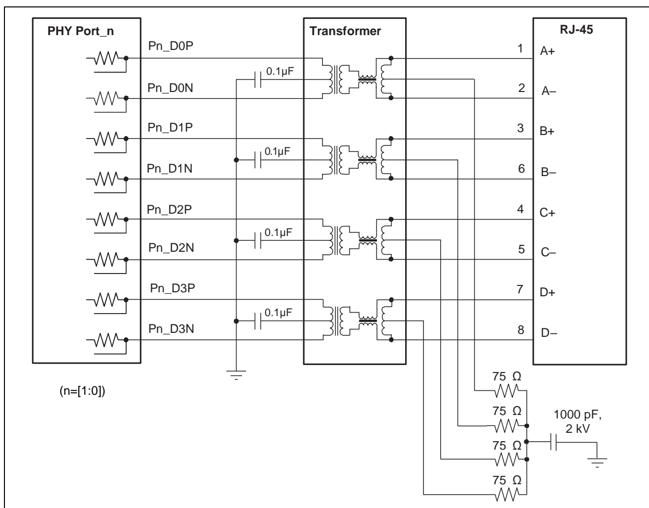
Figure 2.1 Media Interface
