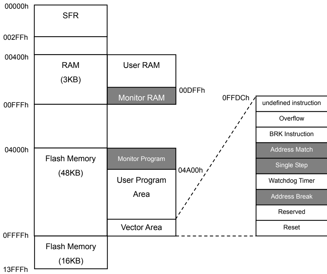
Figure 4 shows the Memory Map of R8C/Tiny On-chip Flash Memory (64KB version).
