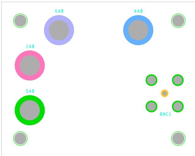
Figure 6. Silk Screen Bottom
