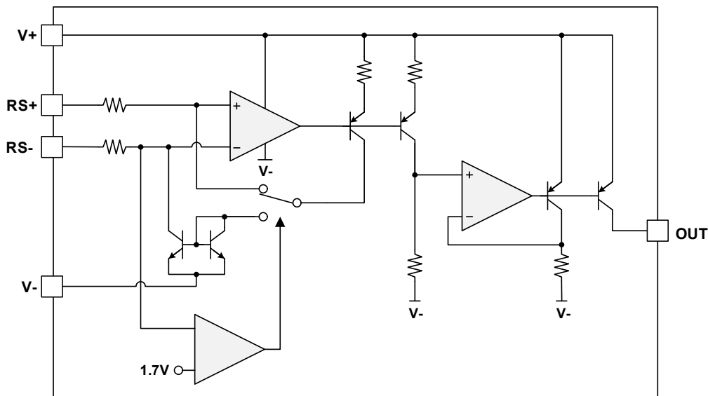
Figure 1. ISL73100SEHEV1Z Block Diagram
