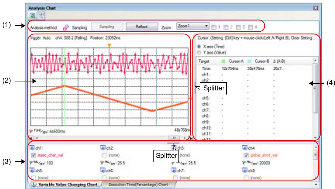
Figure A.9 Analysis Chart Panel: [Variable Value Changing Chart] Tab
