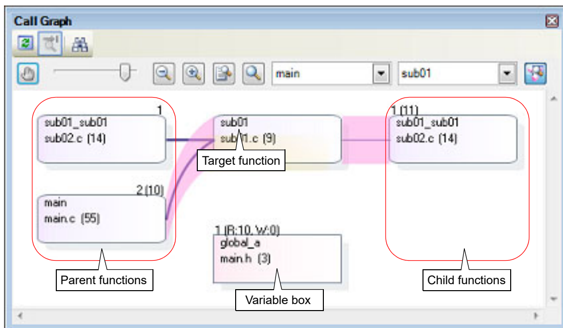
Figure A.17 Call Graph Panel (Details View)
