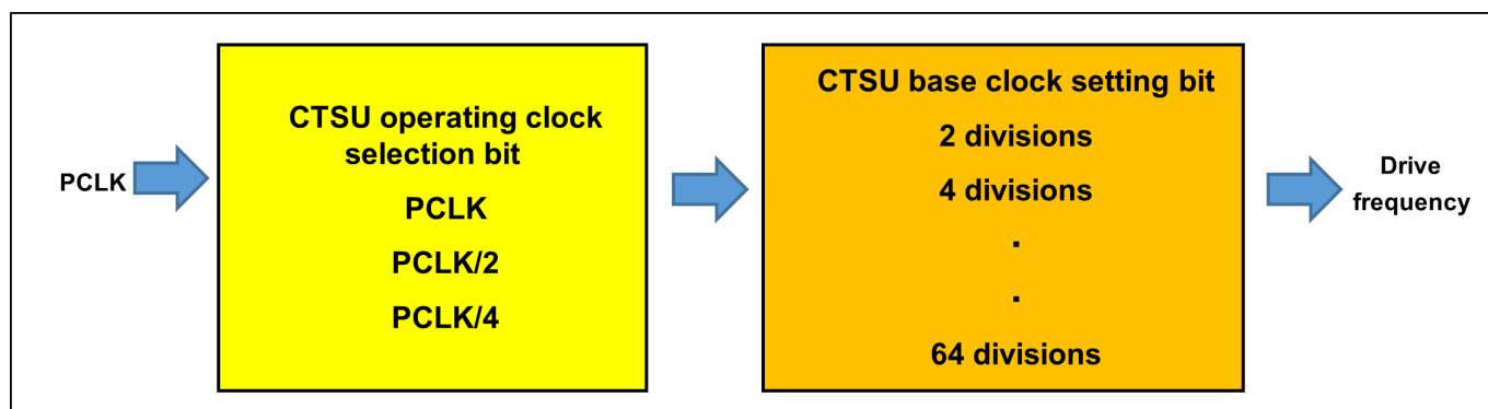
Figure 150: Drive Frequency Settings
