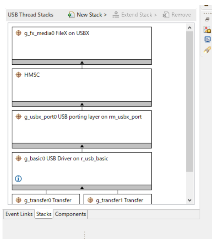
Figure 217: FileX on USBX Stack
