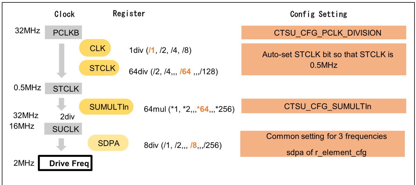
Figure 152: Drive Frequency Settings
