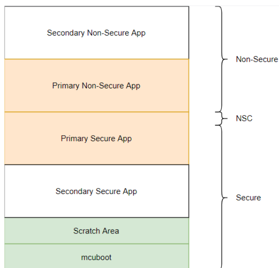
Figure 204: MCUboot Memory Map (TrustZone)
