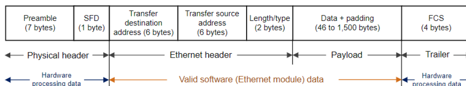
Figure 162: Frame Format Image
