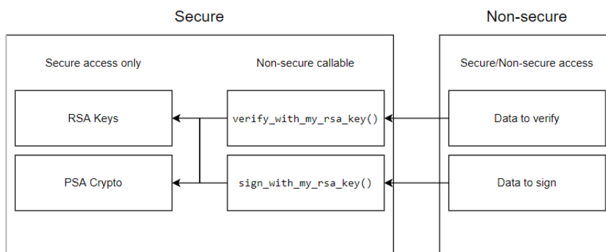
Figure 205: PSA Crypto Non-secure callable example
