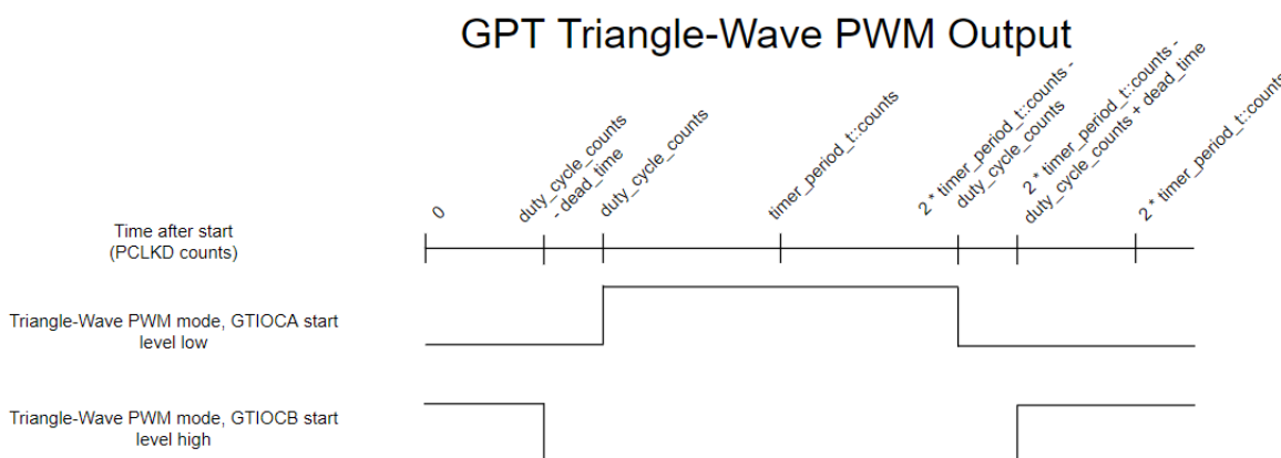
Figure 169: GPT Triangle-Wave PWM Output
