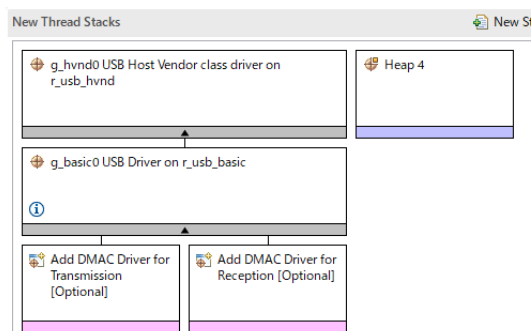
Figure 190: USB Host Vendor Class Stack
