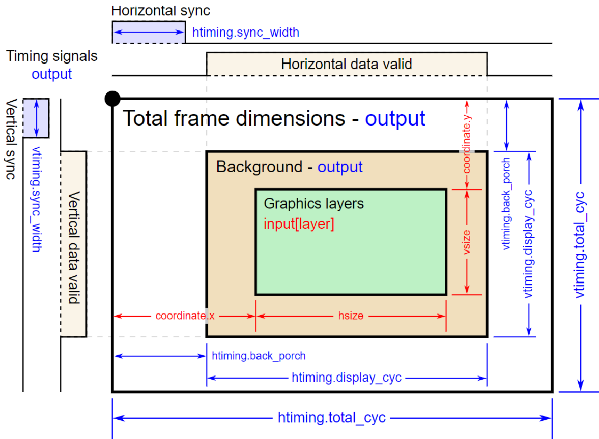
Figure 165: GLCDC layers and timing
