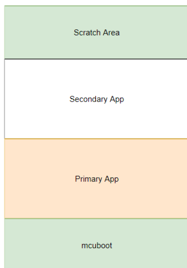
Figure 203: MCUboot Memory Map
