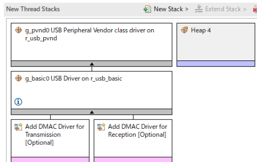
Figure 199: USB Peripheral Vendor Class Stack
