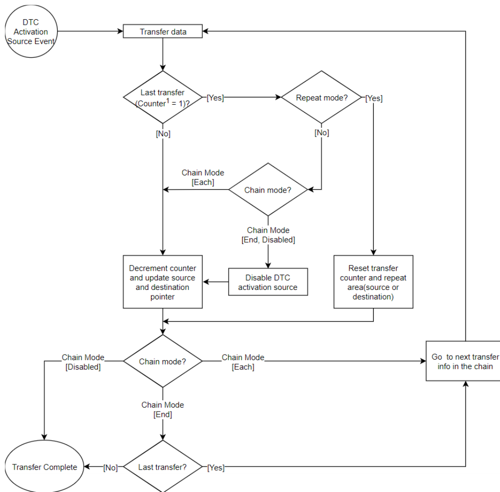
Figure 159: DTC Transfer Flowchart
