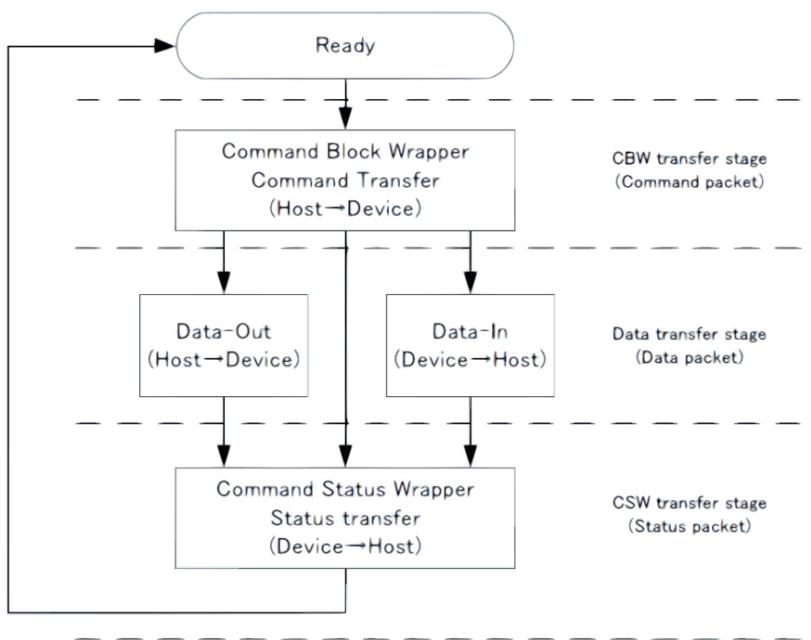
Figure 196: BOT protocol Overview
