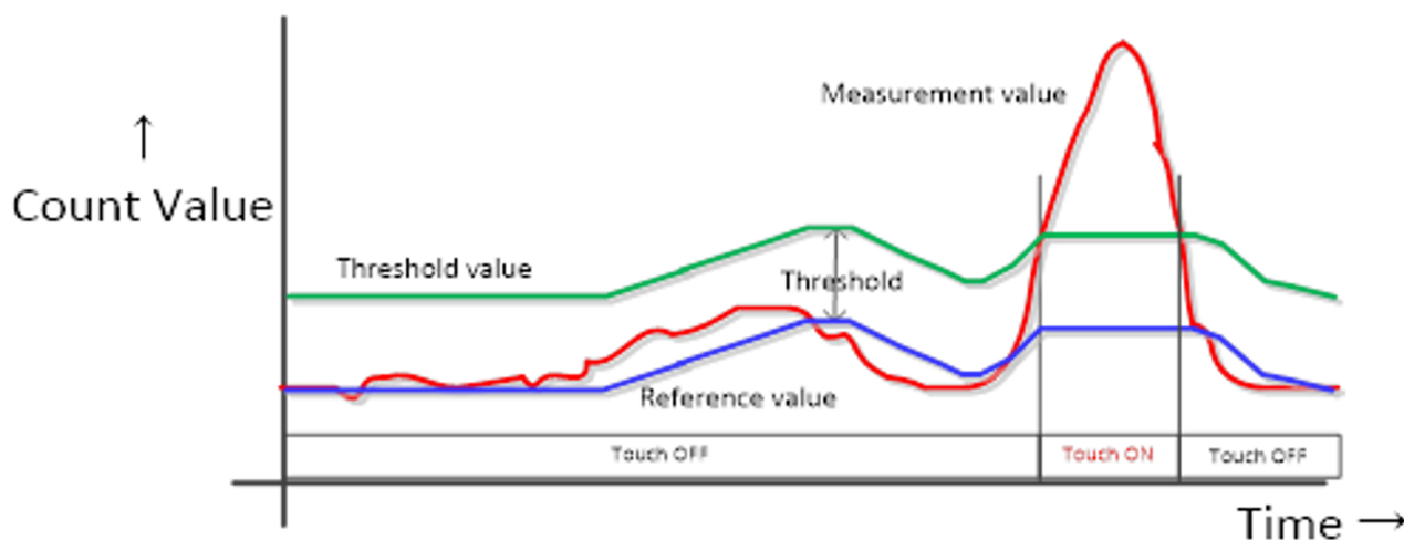
Figure 206: Button Touch Determination
