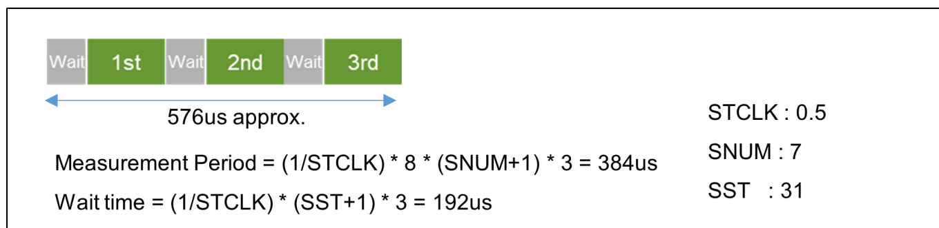
Figure 155: Self-capacitance Measurement Period (CTS2)
