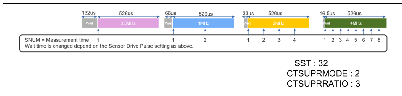
Figure 154: Self-capacitance Measurement Period (CTS1)
