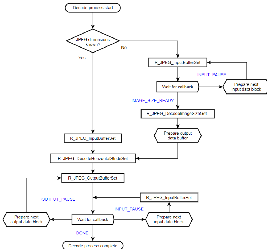
Figure 172: JPEG Decode Operational Flow
