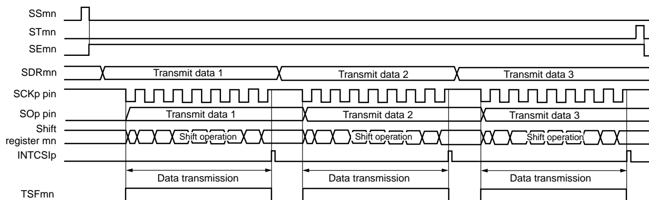
Figure 12-52. Timing Chart of Slave Transmission (in Single-Transmission Mode) (Type 1: DAPmn = 0, CKPmn = 0)
