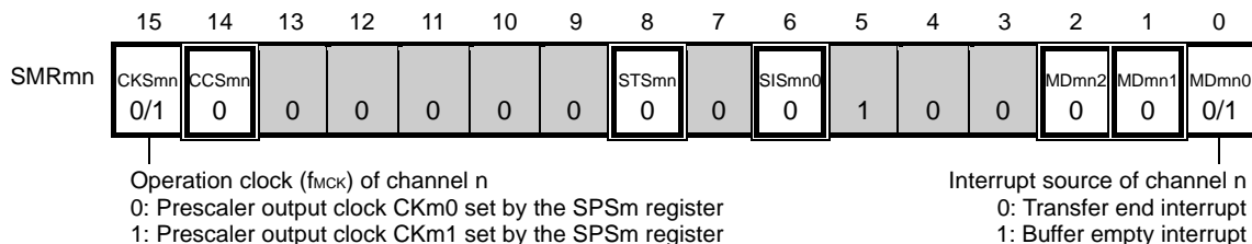
Figure 12-32. Example of Contents of Registers for Master Reception of Simplified SPI (CSI00, CSI01, CSI10, CSI11, CSI20, CSI21) (1/2)
