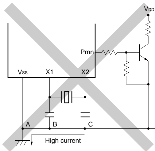
(f) Current flowing through ground line of oscillator (potential at points A, B, and C fluctuates)
