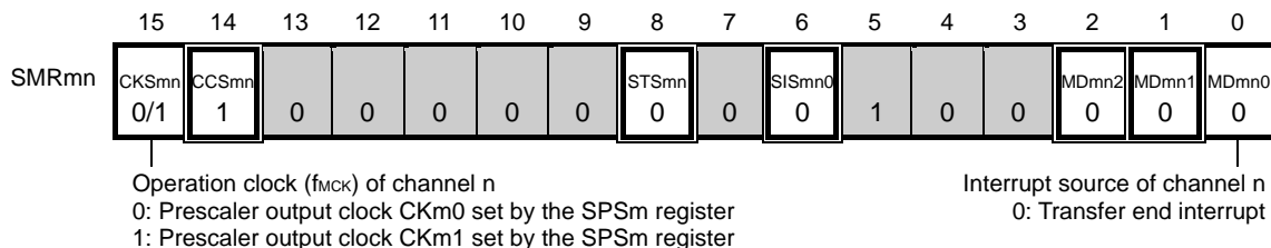
Figure 12-56. Example of Contents of Registers for Slave Reception of Simplified SPI (CSI00, CSI01, CSI10, CSI11, CSI20, CSI21)
