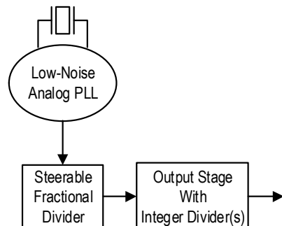
Figure 23. Free-Running Synthesizer Operation
