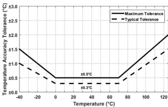
Figure 11. HS4004 Temperature Sensor Accuracy Tolerance
