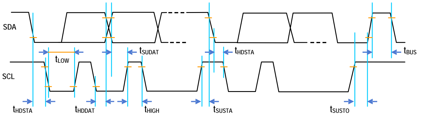
Figure 12. Timing Diagram
