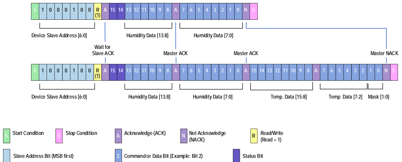
Figure 16. Data Fetch
