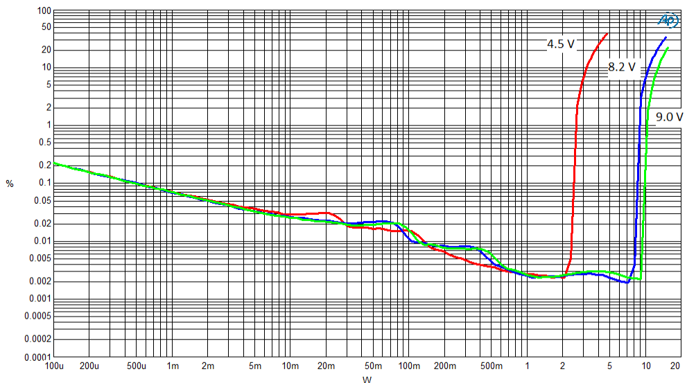
Figure 4: THD versus output power (4 Ω + 33 μH)
