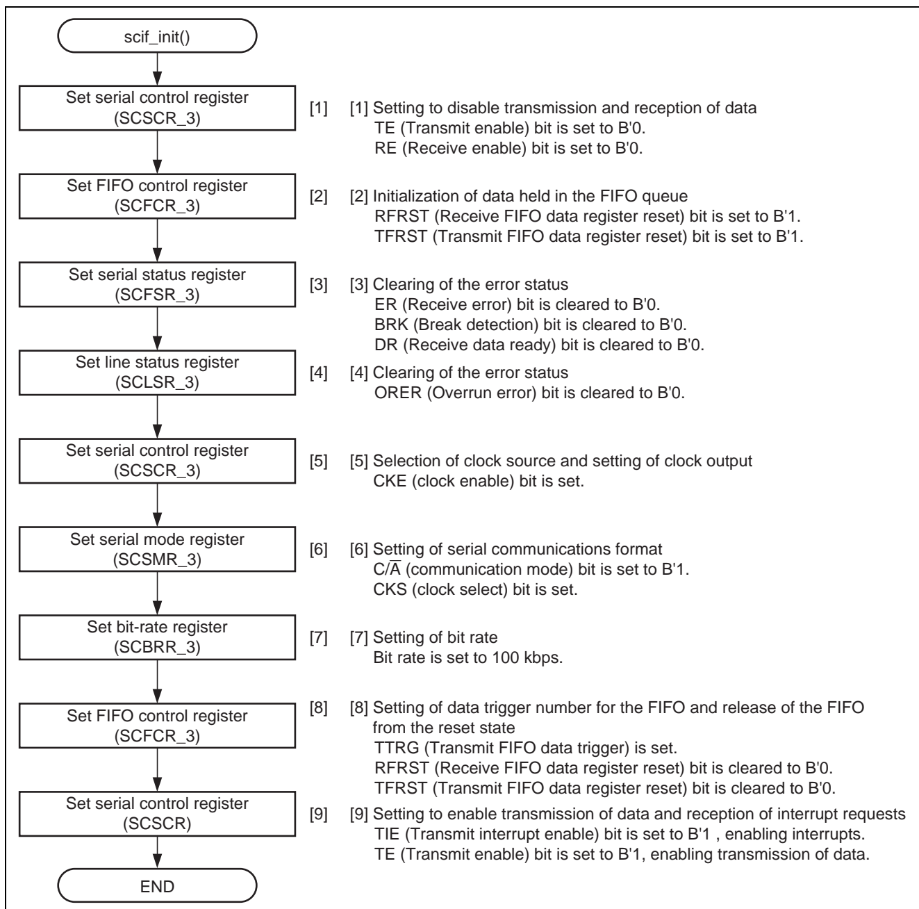
Figure 7 Flow for Initialization of Data Transmission in Clock-Synchronous Mode
