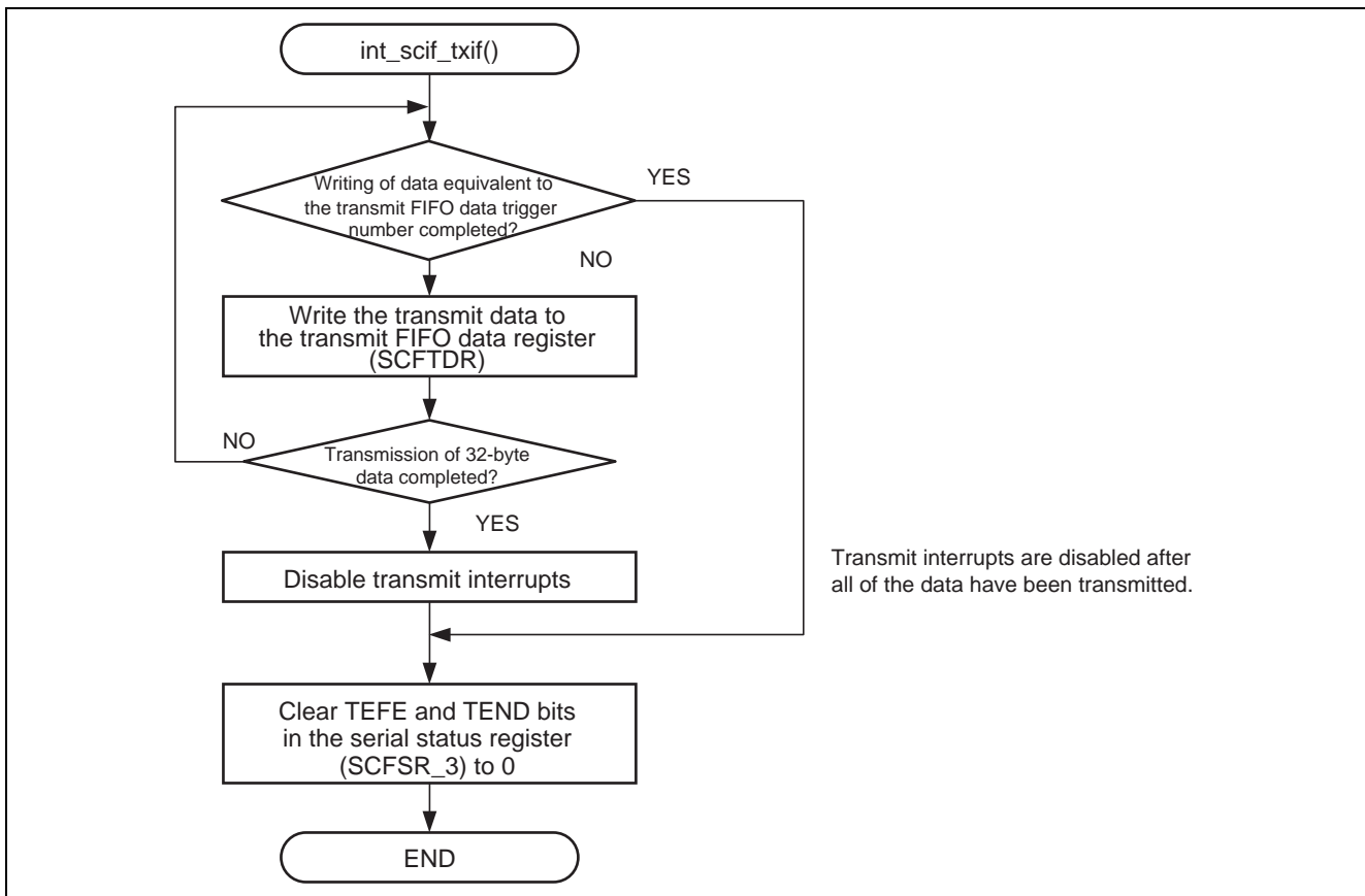
Figure 8 Flow for Handling of Transmit Interrupts in Clock-Synchronous Mode
