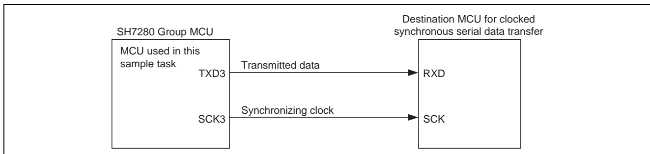
Figure 1 Connection Example for Transmission by the SCIF in Clock-Synchronous Mode
