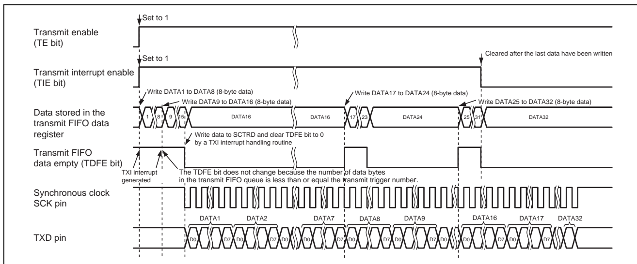
Figure 3 Operations for Data Transmission
