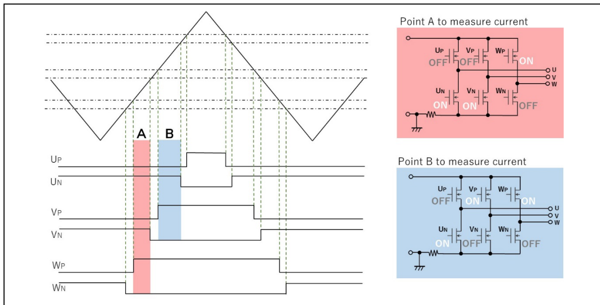
Figure 3-3 The wave form of PWM (in case of duty pattern W > V > U )
