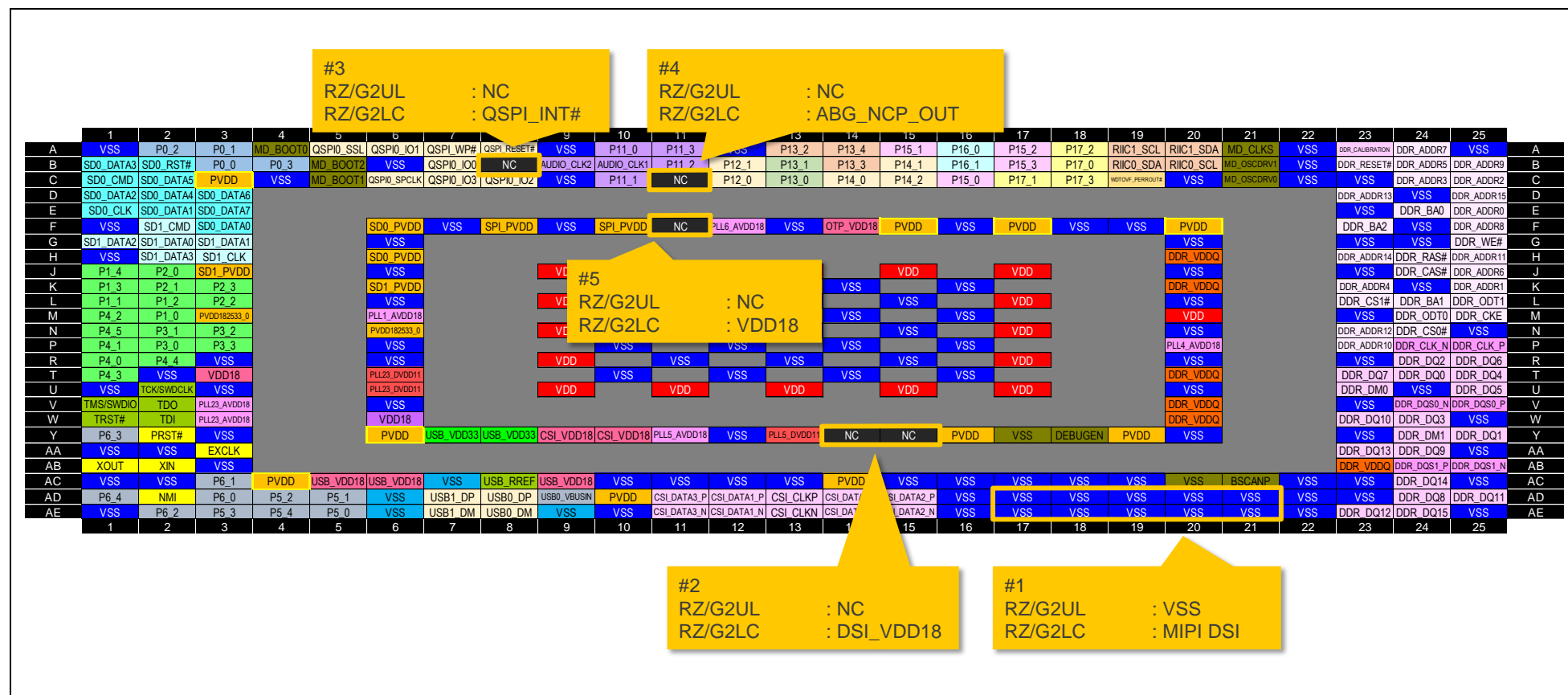
Figure 2.2 RZ/G2UL Type-2 ball view
