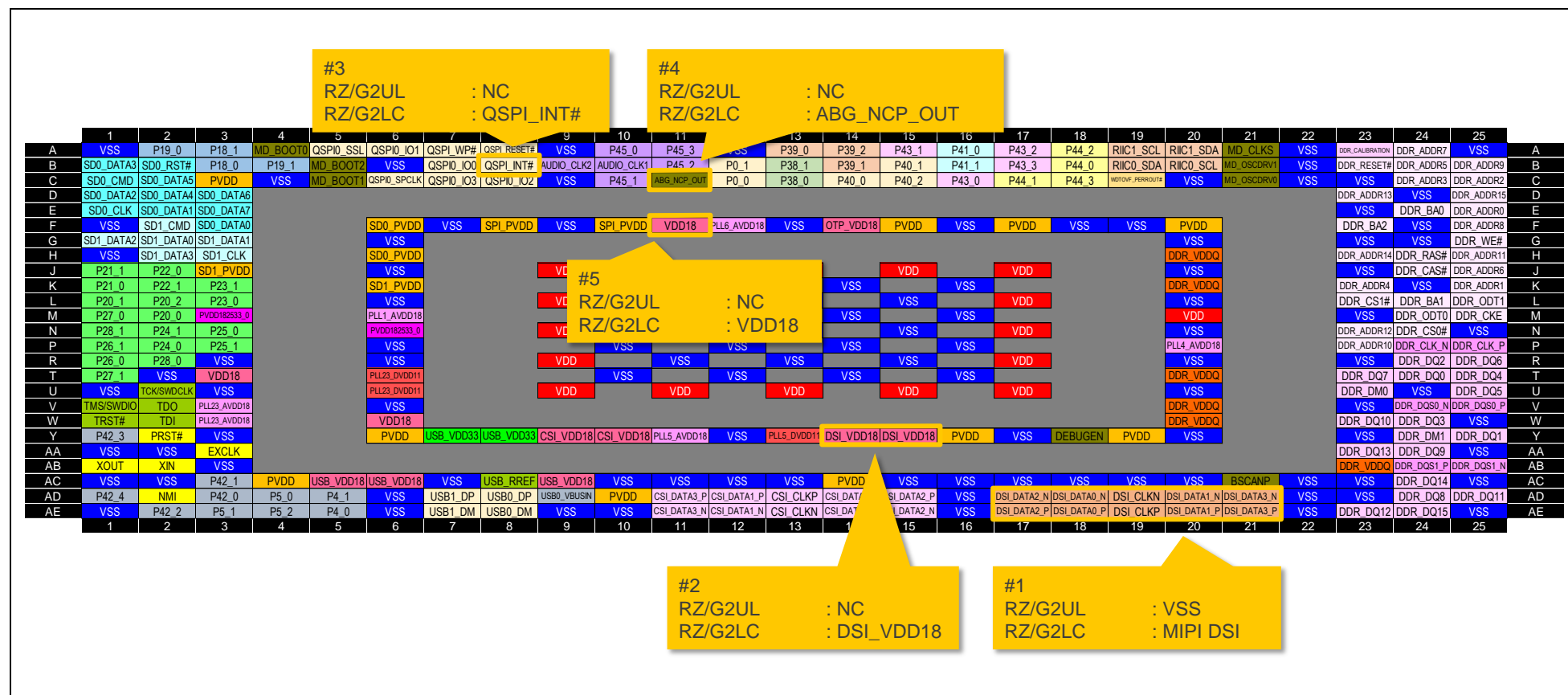
Figure 2.1 RZ/G2LC Ball View
