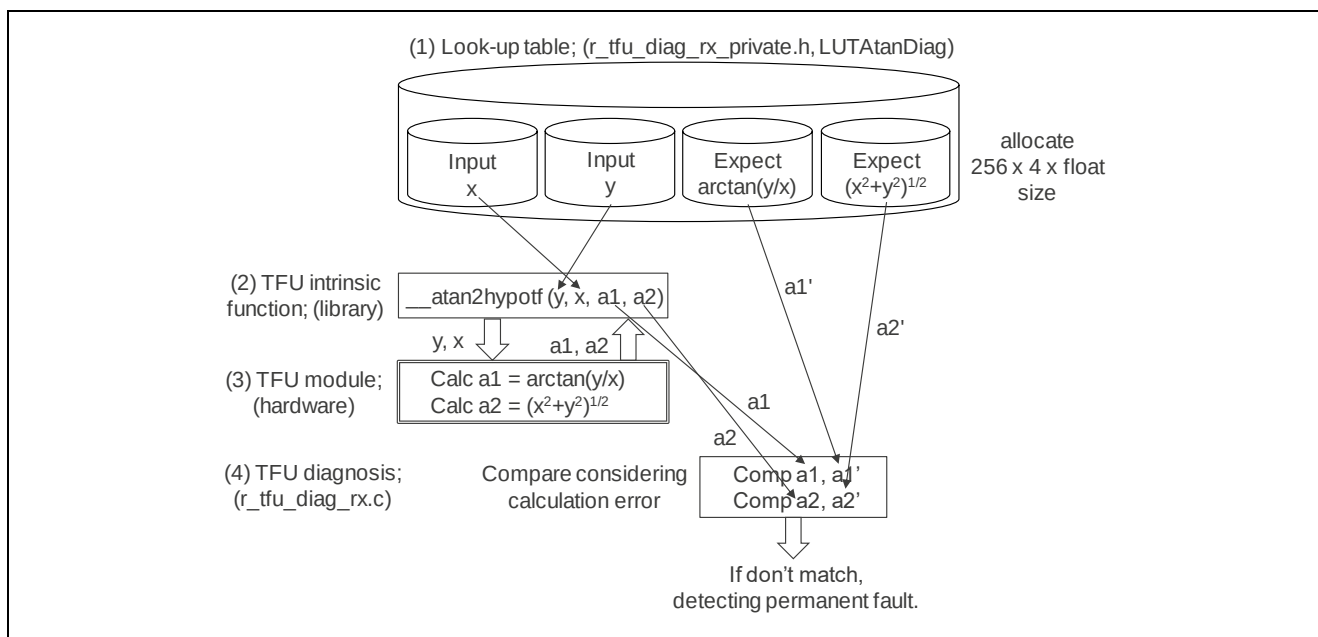
Figure 3.5 Permanent Fault (arctangent &amp; hypotenuse)
