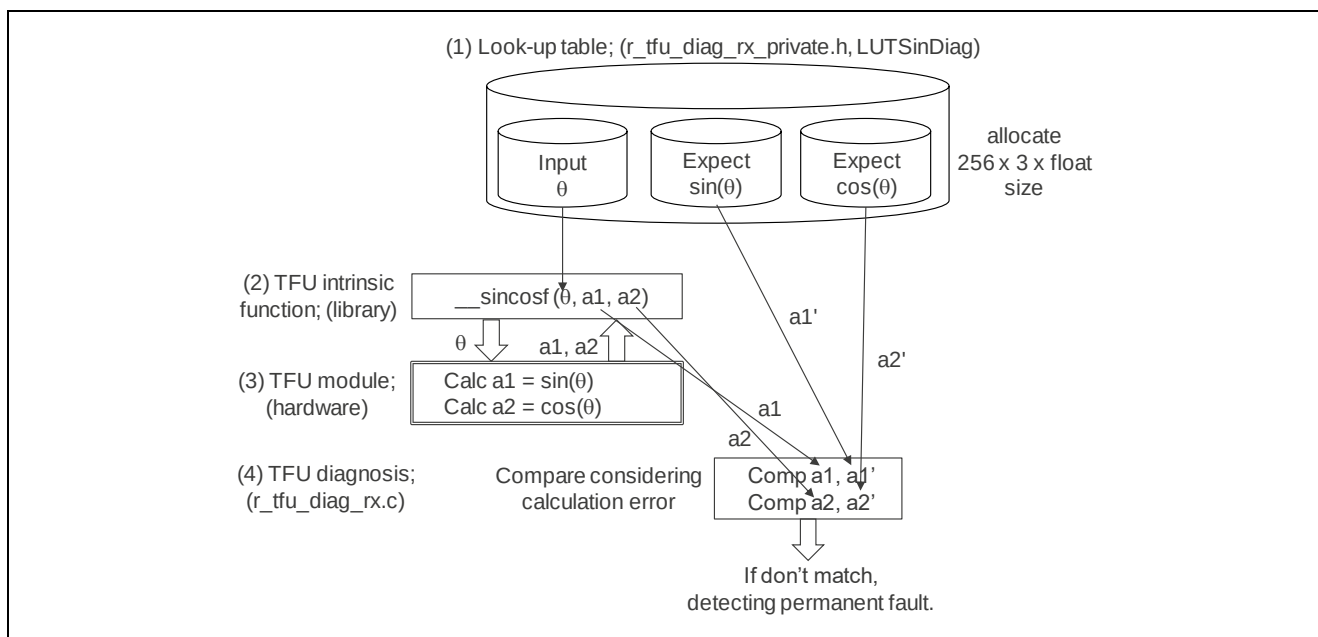
Figure 3.4 Permanent Fault (sine &amp; cosine)
