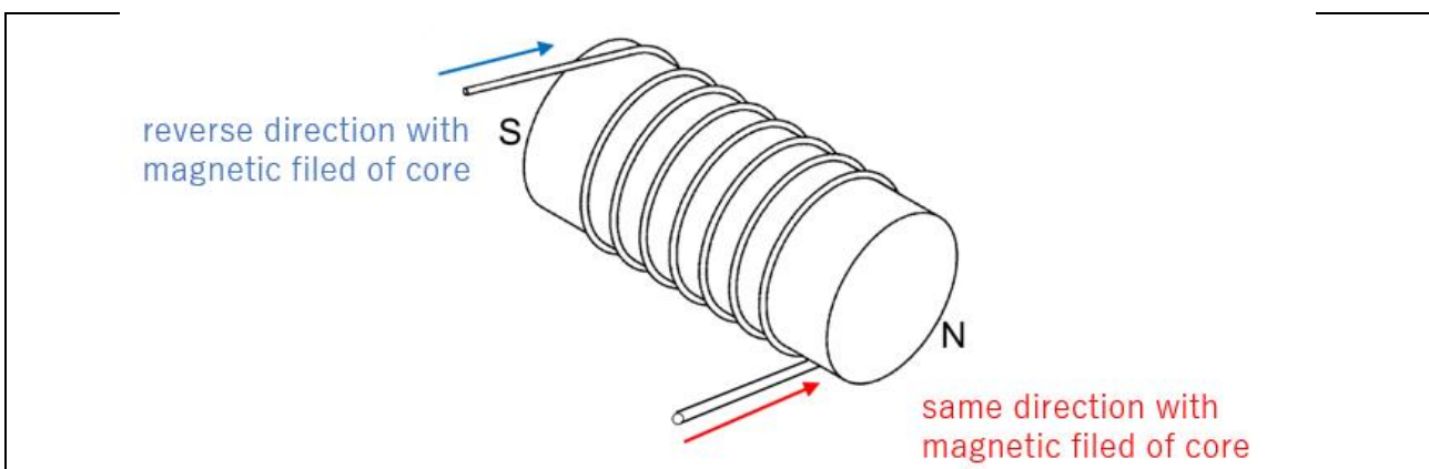
Figure 3-19 Example of magnetic pole wound with coil
