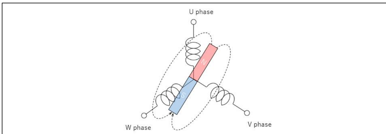
Figure 3-15 Relationship between rotor position and each phase
