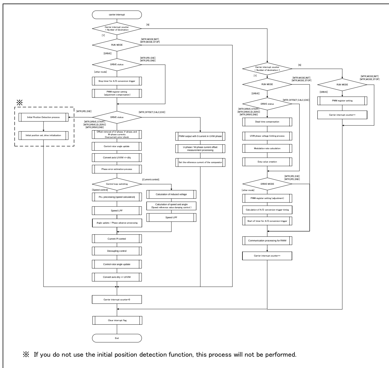
Figure 3-28 Carrier Cycle Interrupt Handling Flowchart
