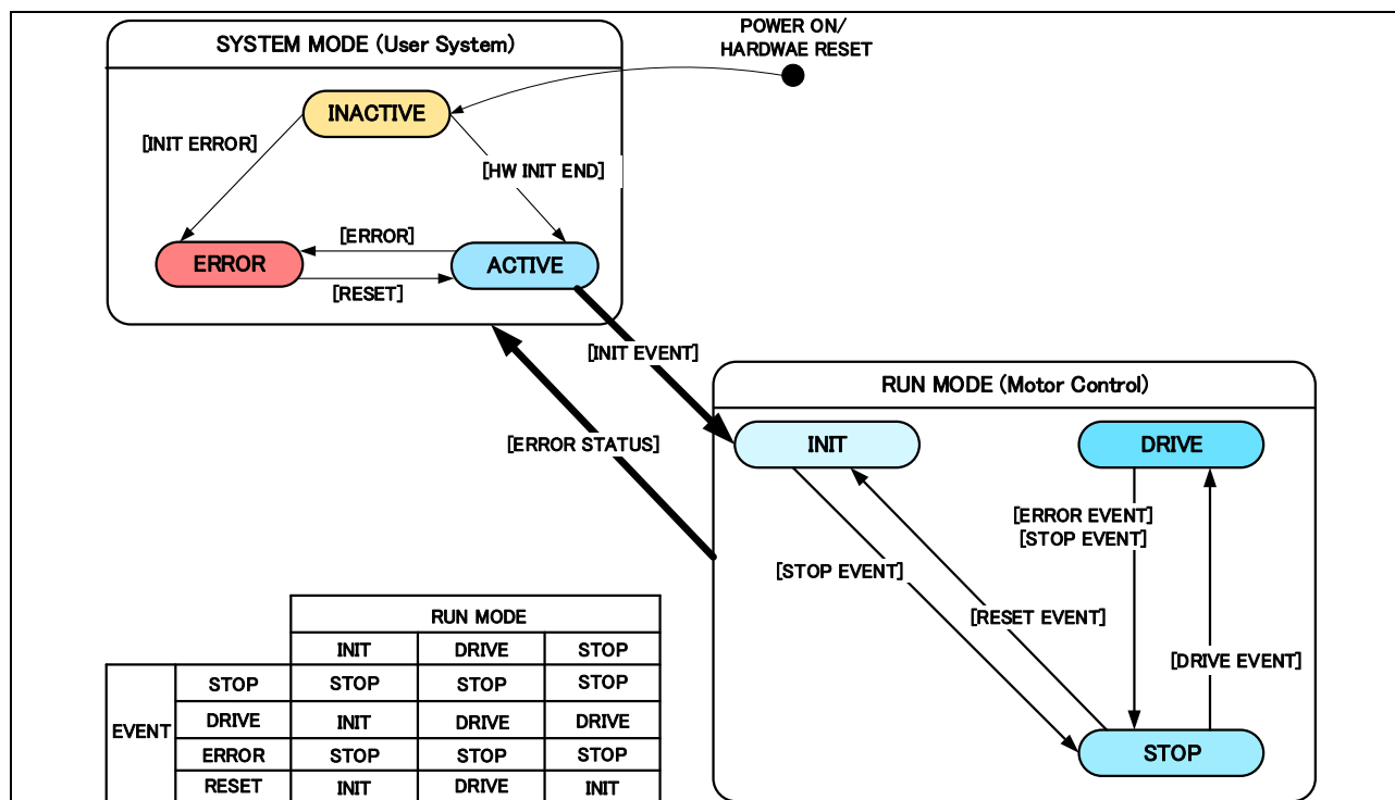
Figure 3-5 State Transition Diagram
