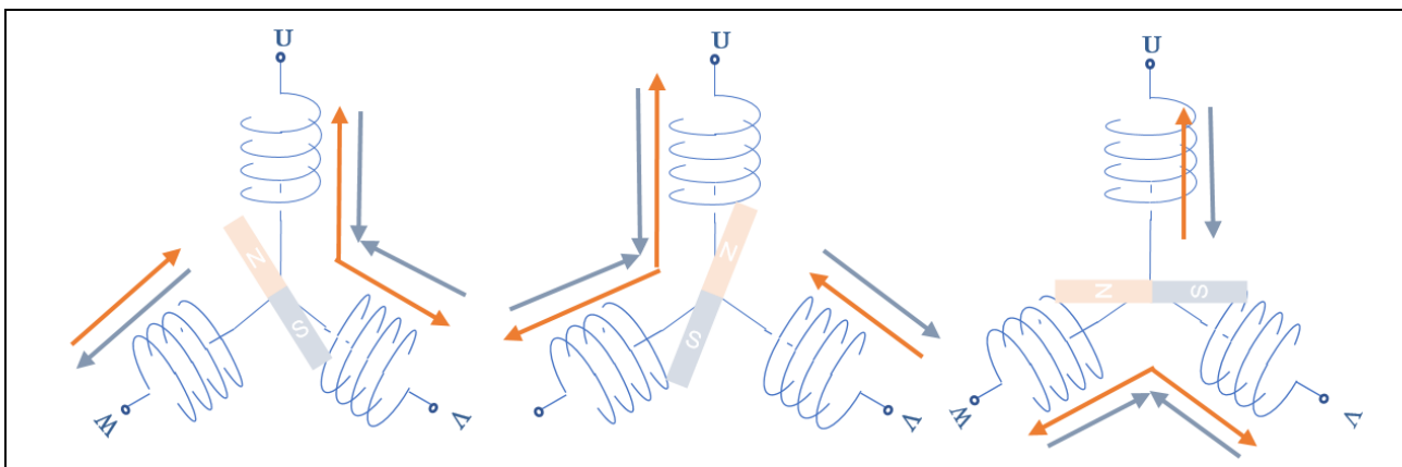
Figure 3-21 Example of applied voltage pattern due to initial position detection using magnetic saturation
