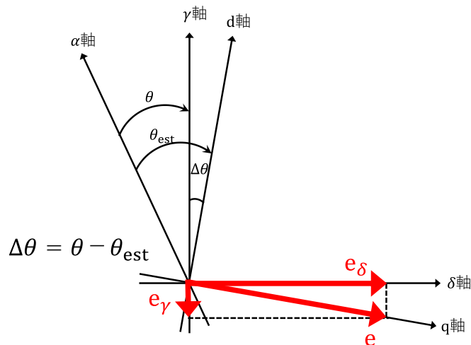
Figure 3-9 Phase Error and \gamma - and \delta -axis Induced Voltage Constituent Elements
