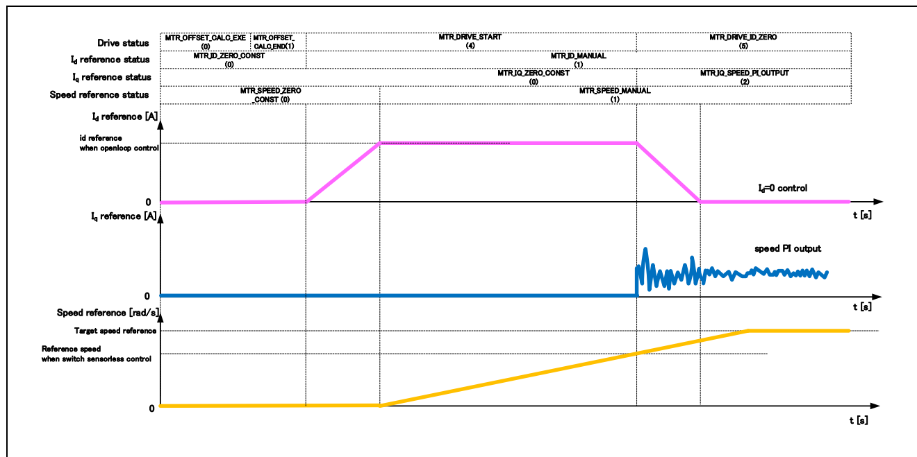
Figure 3-6 Description of Sensorless Speed Control Software Startup Control
