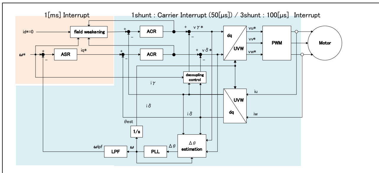
Figure 3-24 Interrupt processing inside control block (during closed loop control)
