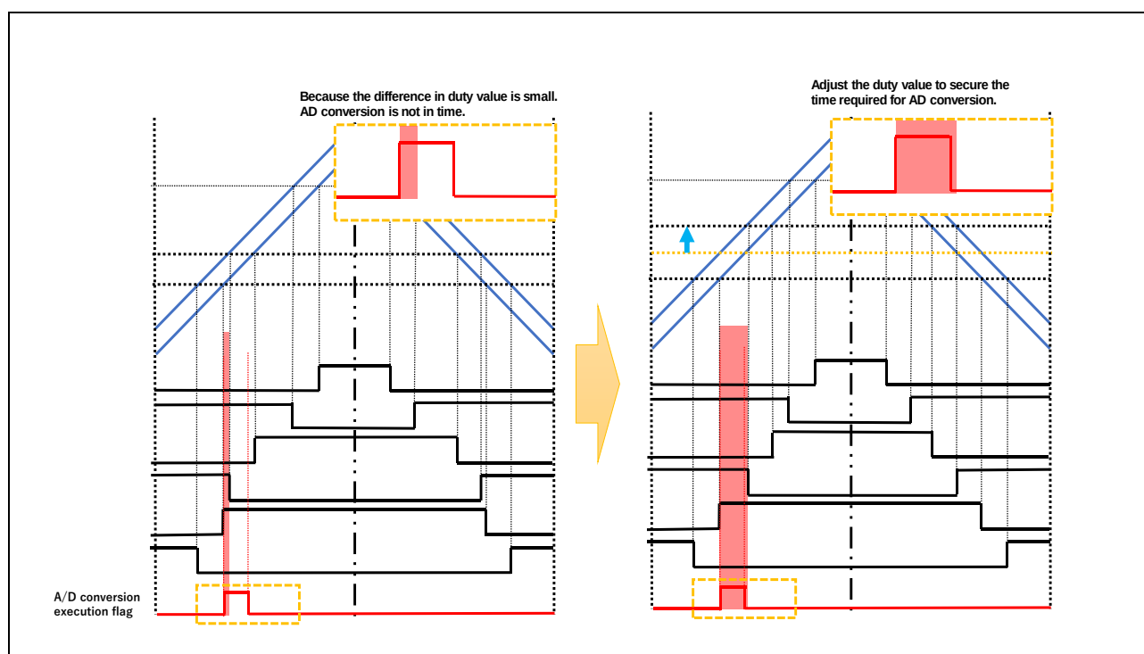
Figure 3-12 Duty adjustment (example)
