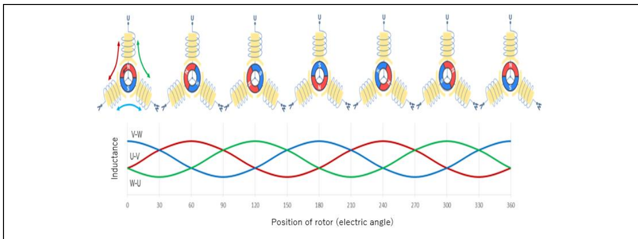
Figure 3-14 Changes in inductance according to rotor position
