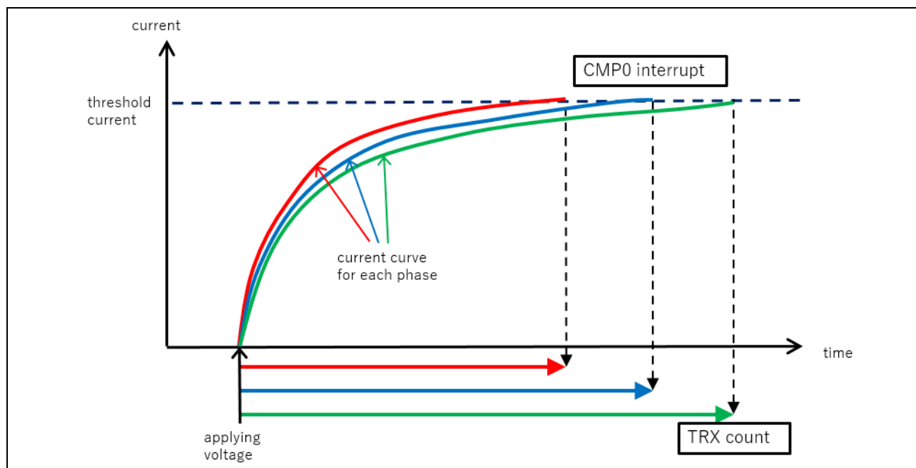
Figure 3-17 Current detection time differential among the 3 Phases
