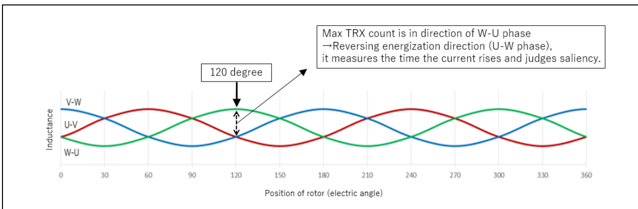
Figure 3-18 Saliency confirmation method
