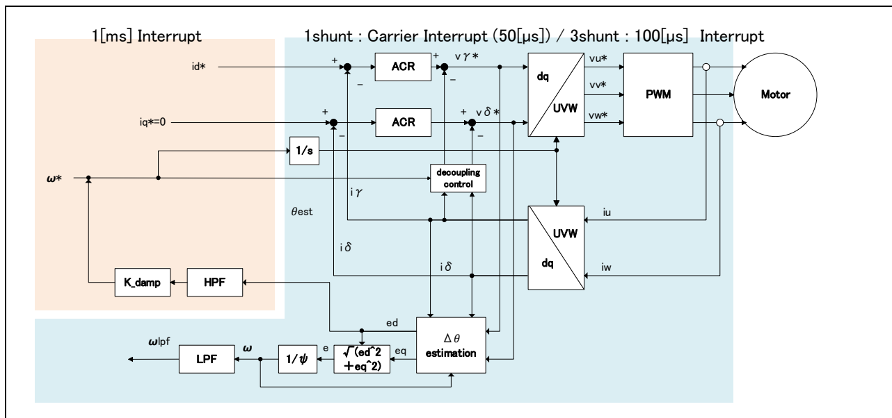
Figure 3-23 Interrupt processing inside control block (during open loop control)
