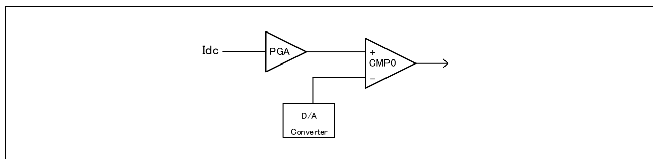
Figure 3-2 Overcurrent detection by CMP0
