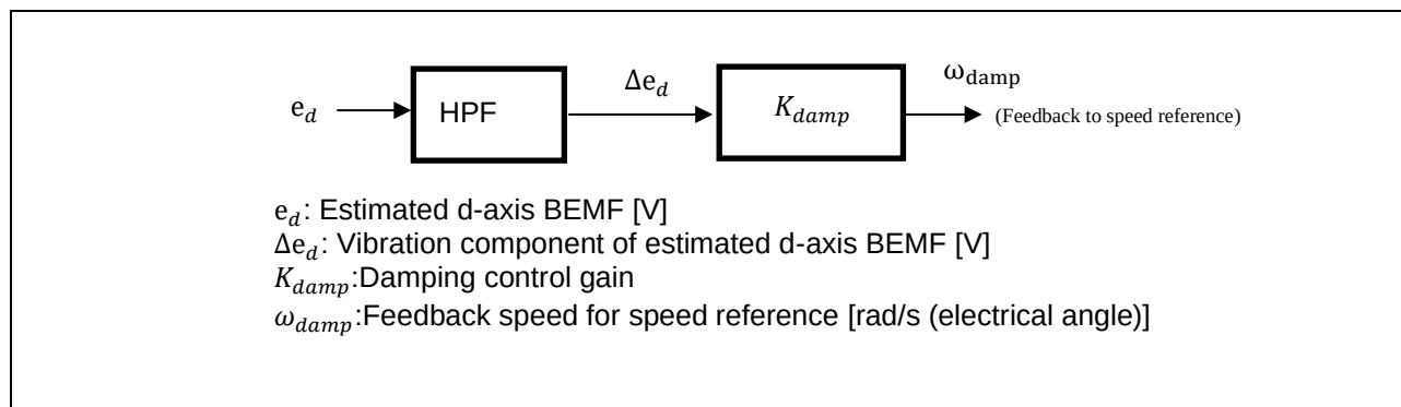
Figure 3-22 Block diagram of the open loop damping control
