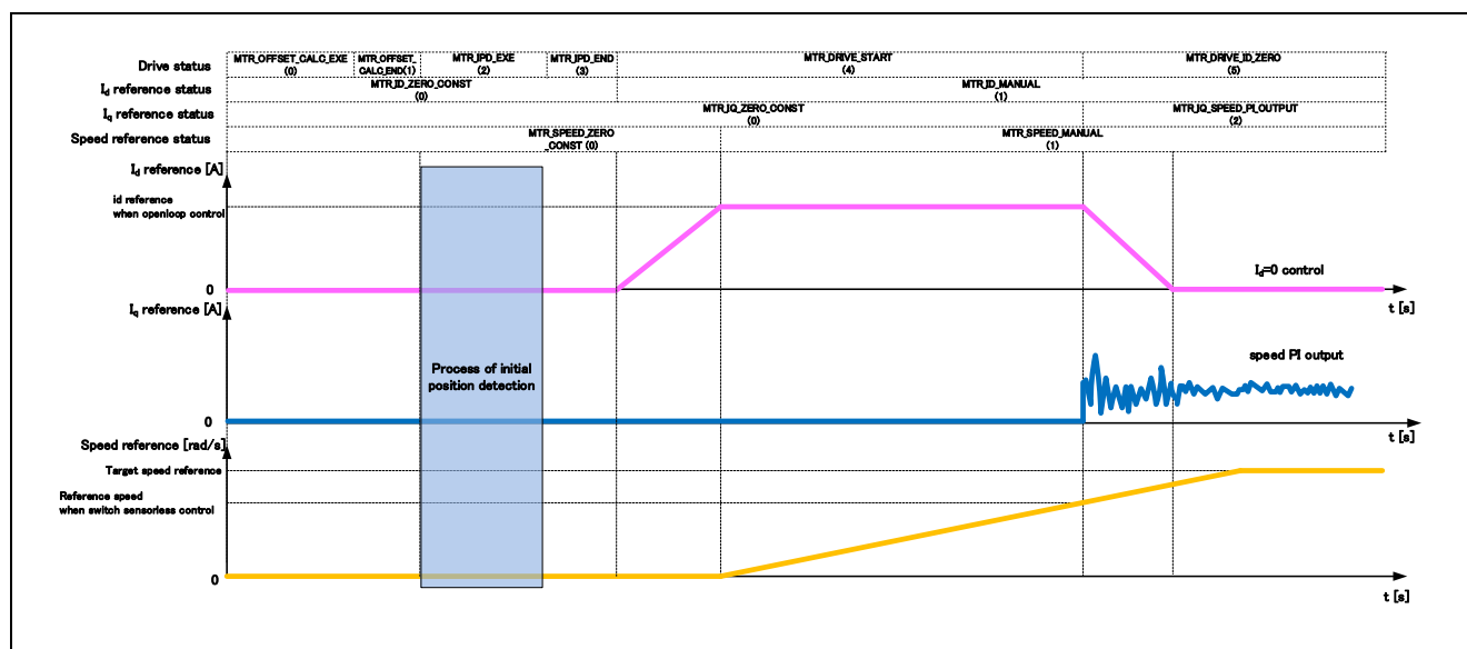
Figure 3-7 Description of Sensorless Speed Control Software Startup Control (IPD processing application)
