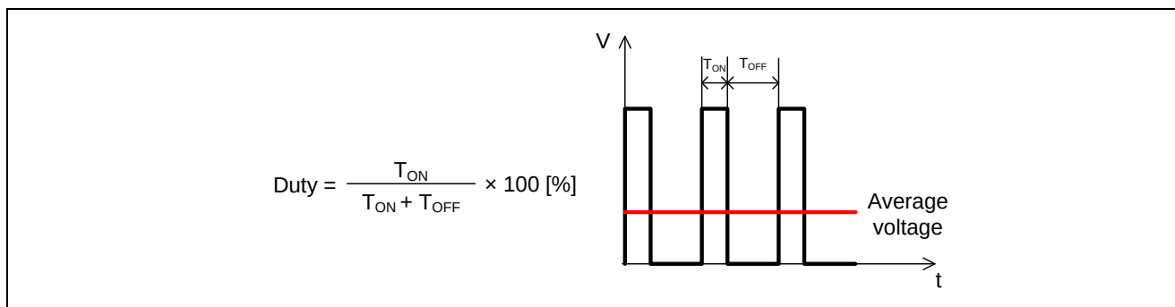
Figure 3-3 PWM Control
