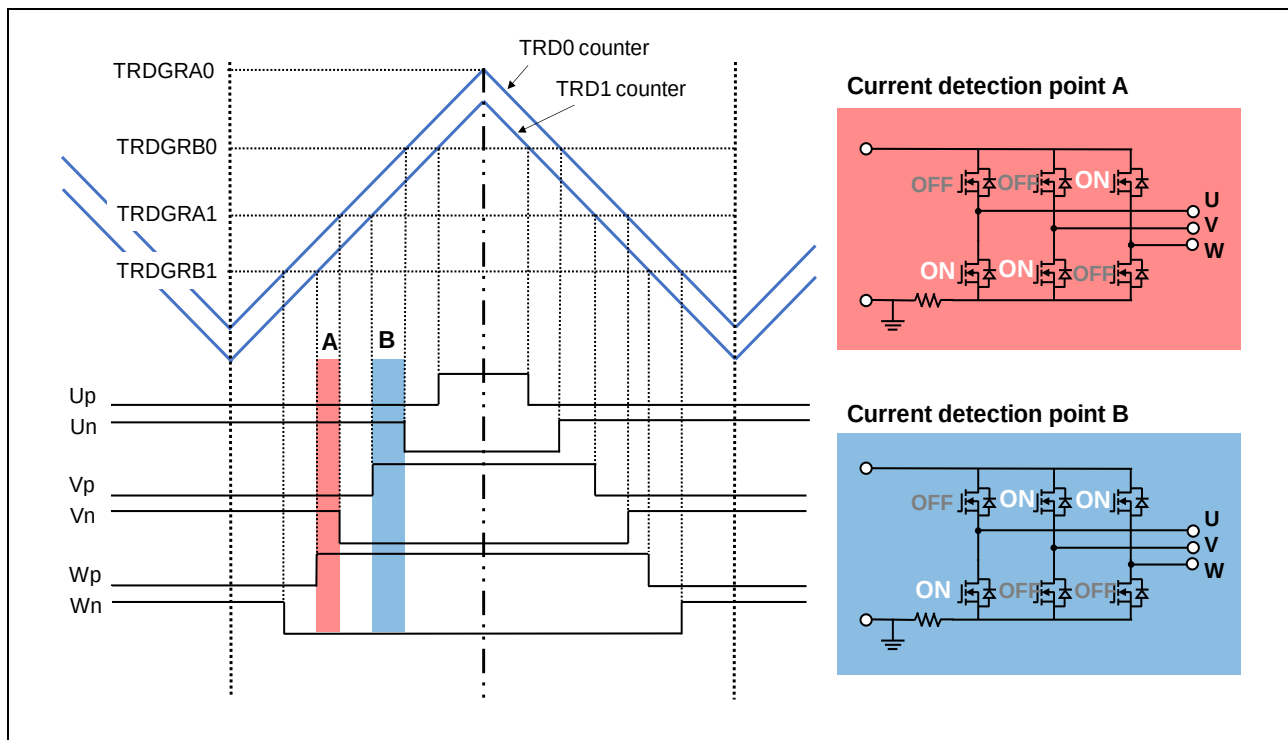
Figure 3-10 Complementary PWM waveform (For example, duty magnitude relation W > V > U ).
