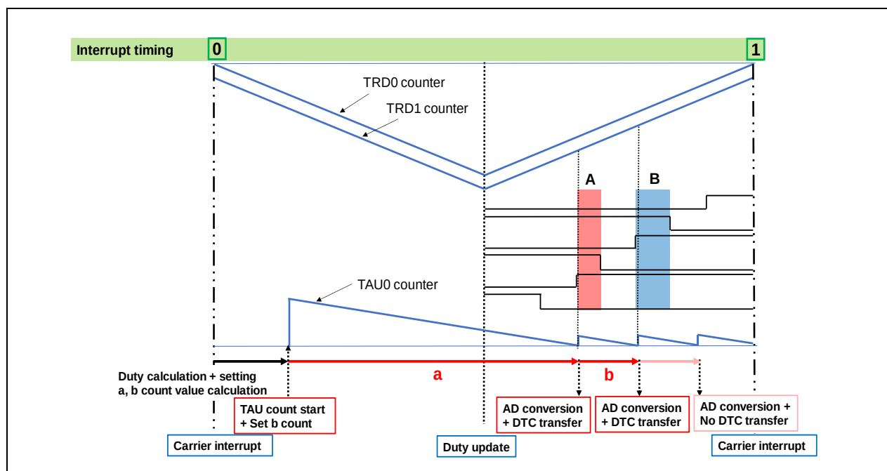
Figure 3-11 Timing of A/D Conversion
