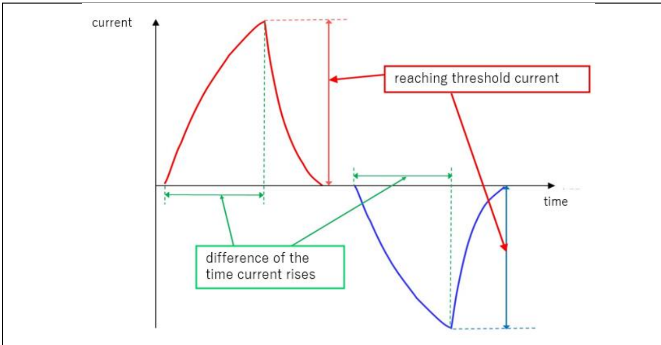
Figure 3-20 Current differential according to direction of applied current
