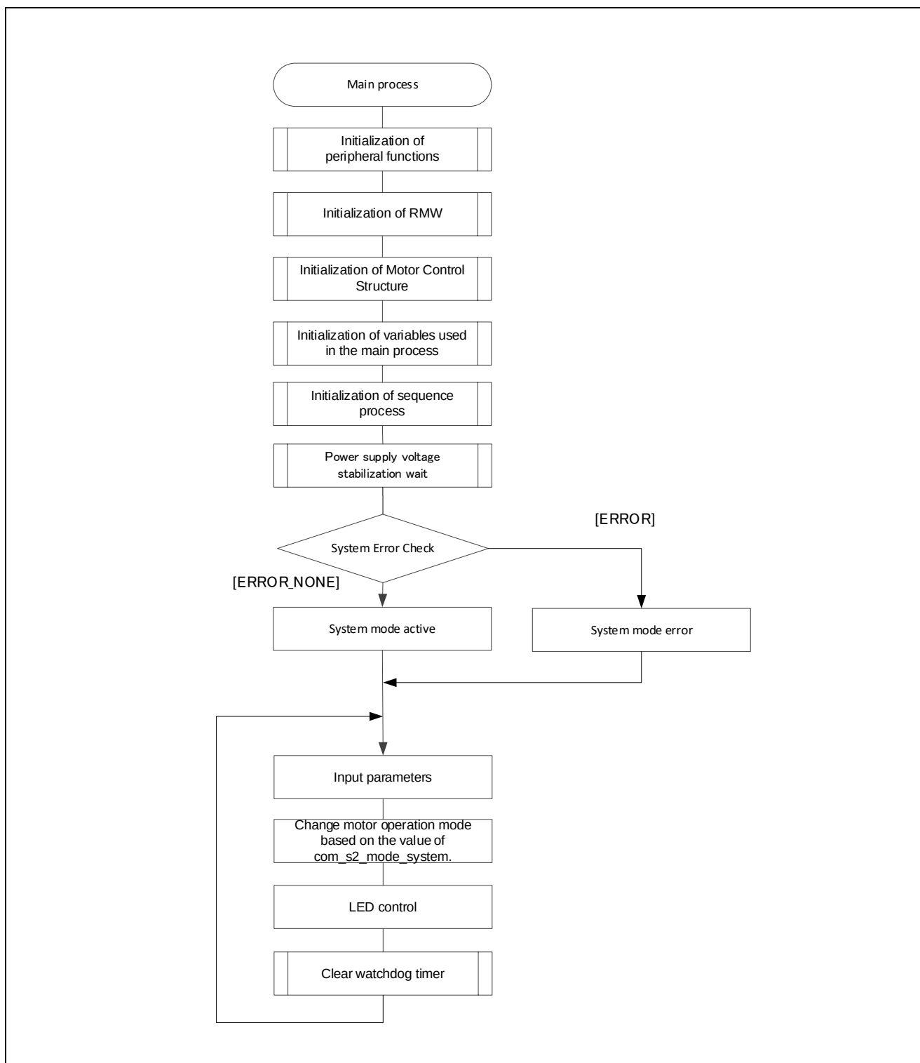
Figure 3-27 Main Process Flowchart
