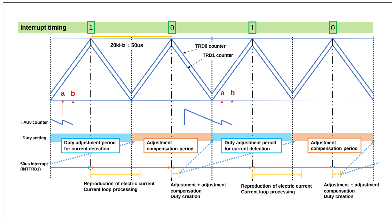
Figure 3-13 Periodic duty adjustment and compensation
