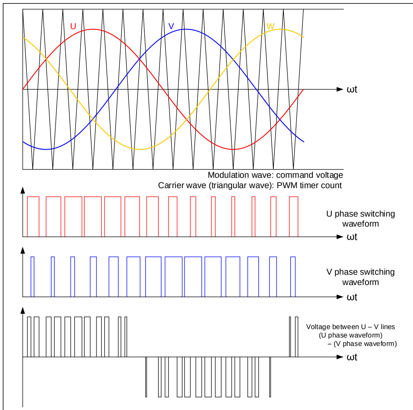
Figure 3-4 Conceptual Diagram of the Triangle Wave Comparison Method
