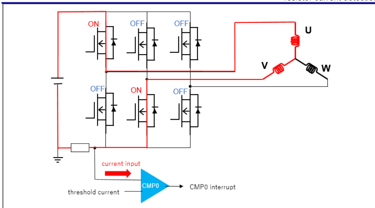
Figure 3-16 Angle detection diagram
