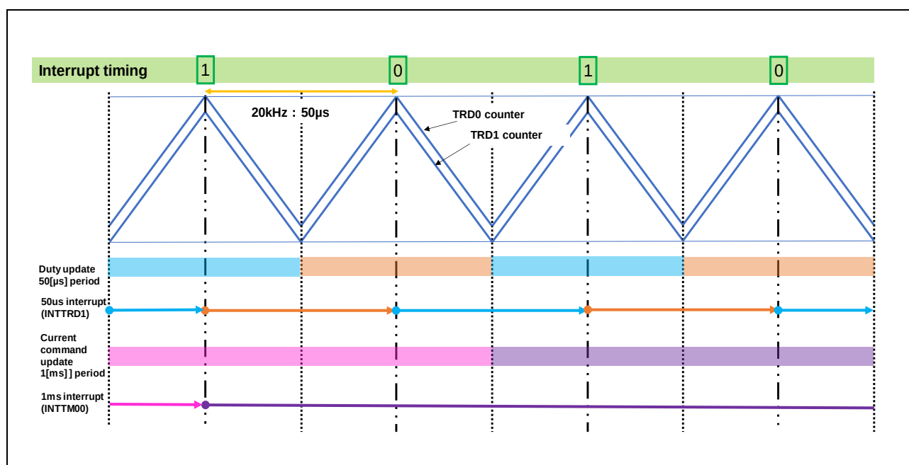
Figure 3-25 Image of interrupt generation and update of output value in 1-shunt mode
