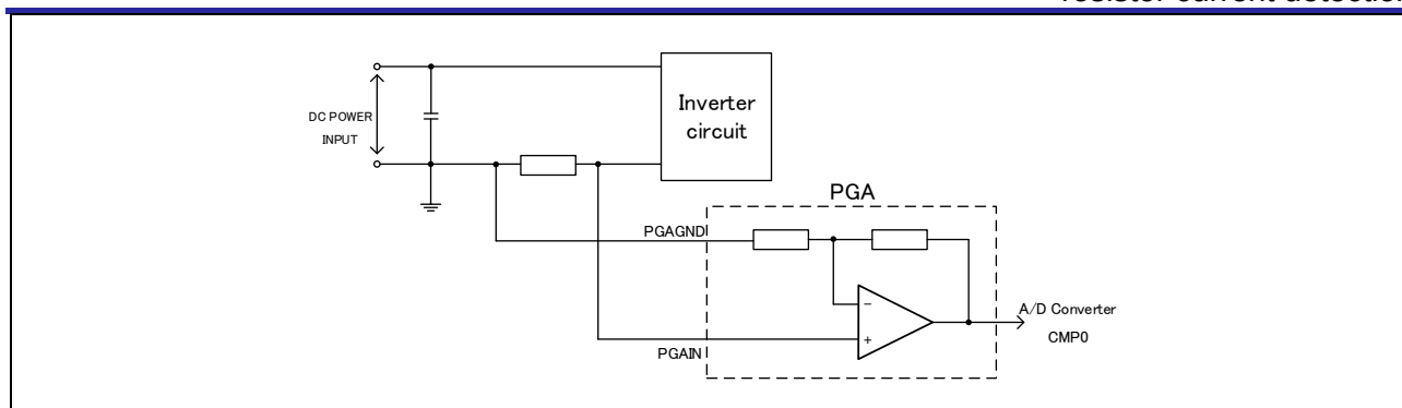
Figure 3-1 Connecting the PGA to the inverter circuit
