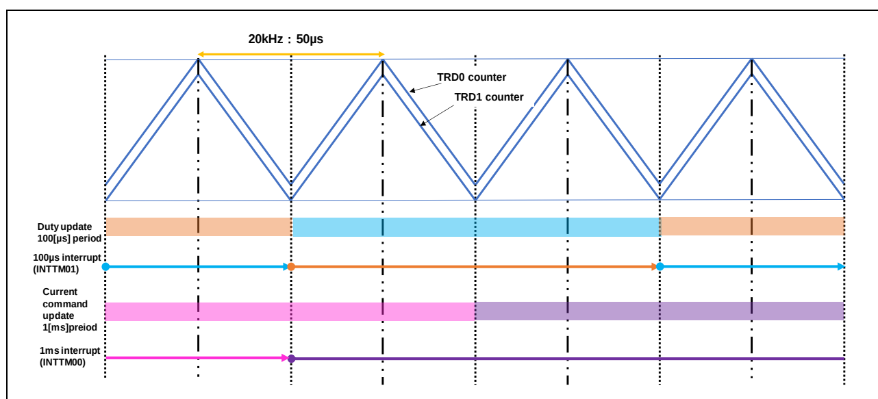
Figure 3-26 Image of interrupt generation and update of output value in 3-shunt mode
