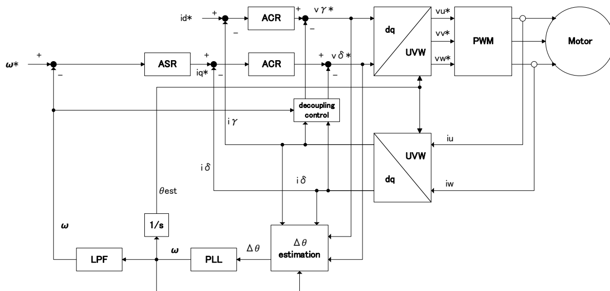
Figure 3-8 Control System Block Diagram
