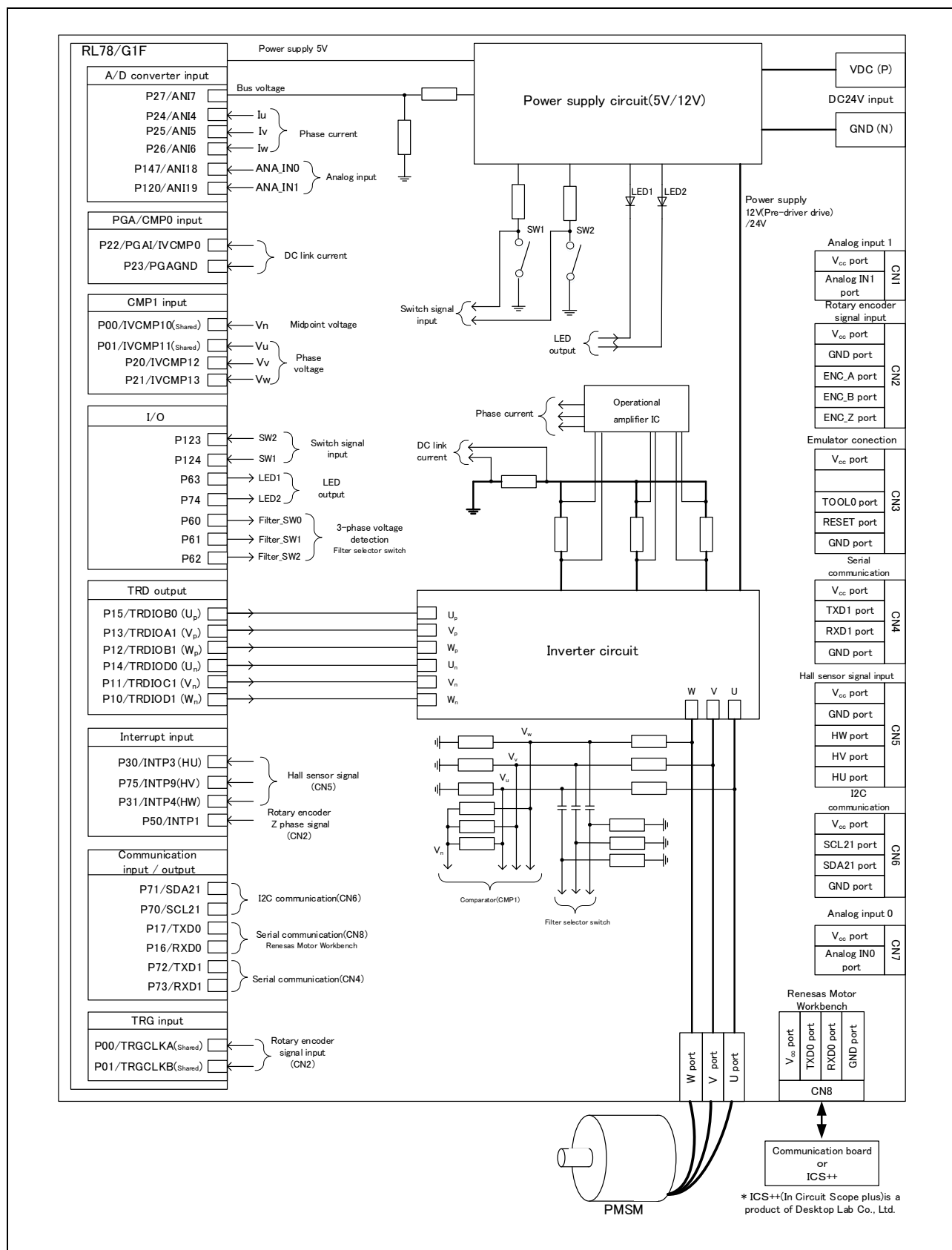
Figure 2-1 Hardware Configuration Diagram
