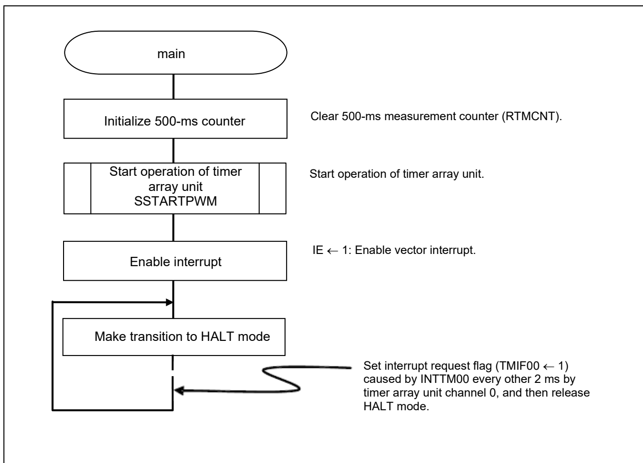
Figure 5.7 Main Processing
