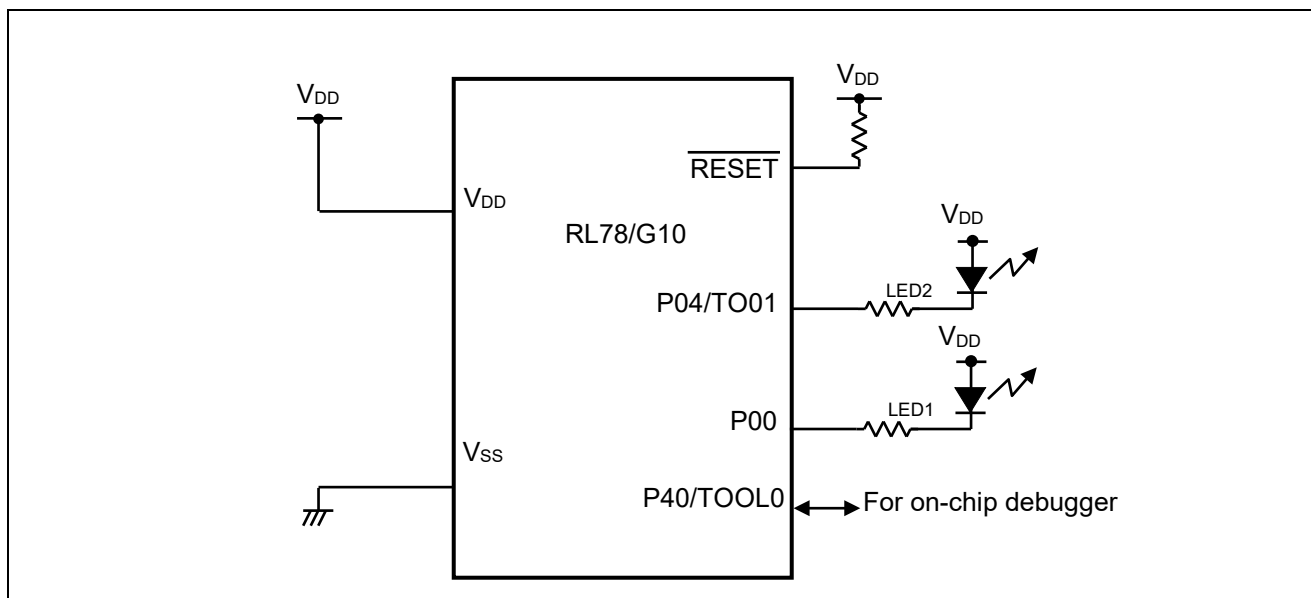
Figure 4.1 Hardware Configuration
