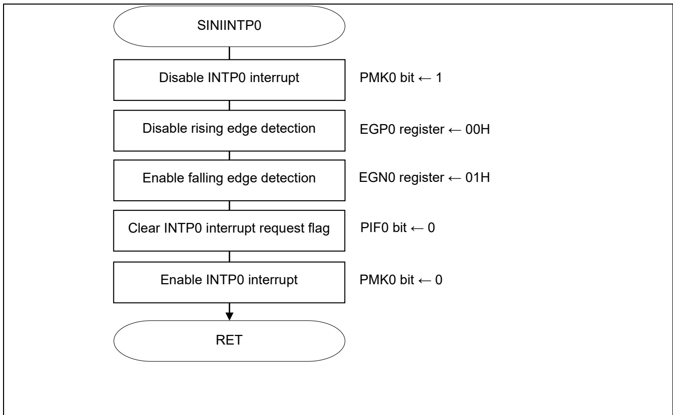
Figure 5.5 INTP0 Initialization
