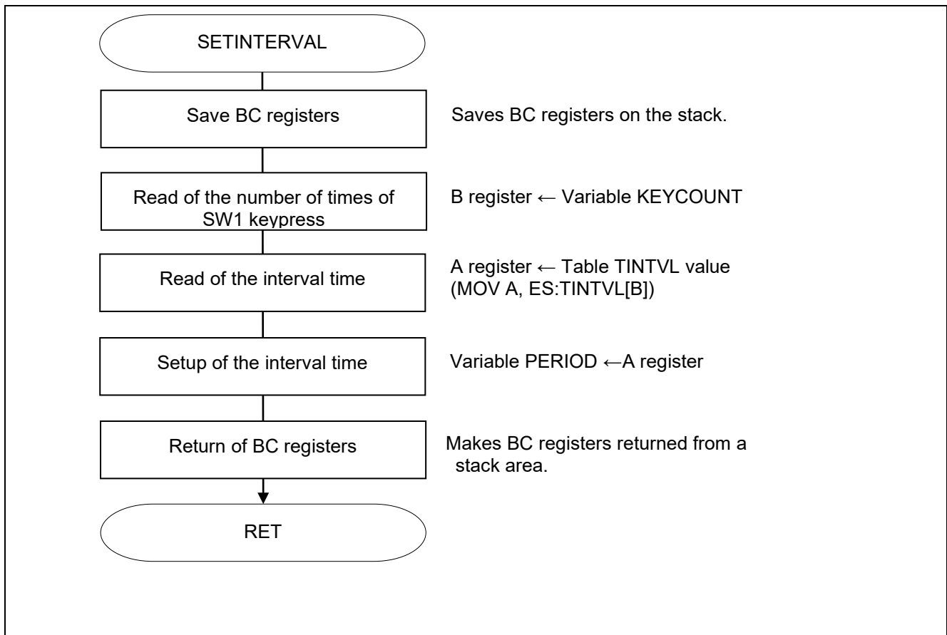
Figure 5.8 Interval Setup
