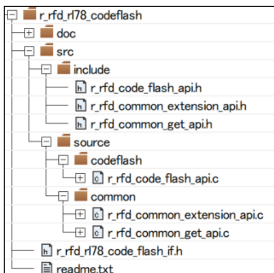
The developed r_rfd_rl78_codeflash folder
