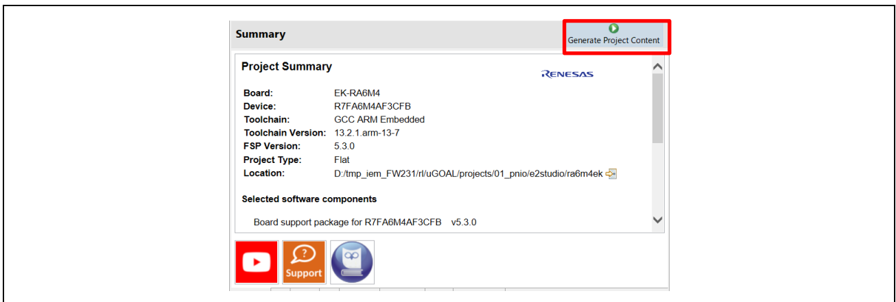
Figure 3.9 Generate code
