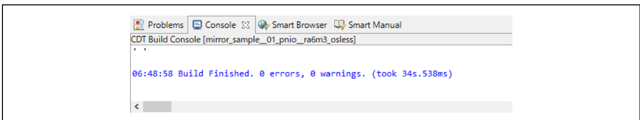
Figure 3.11 Build finished
