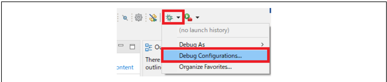
Figure 3.12 Debug Configurations
