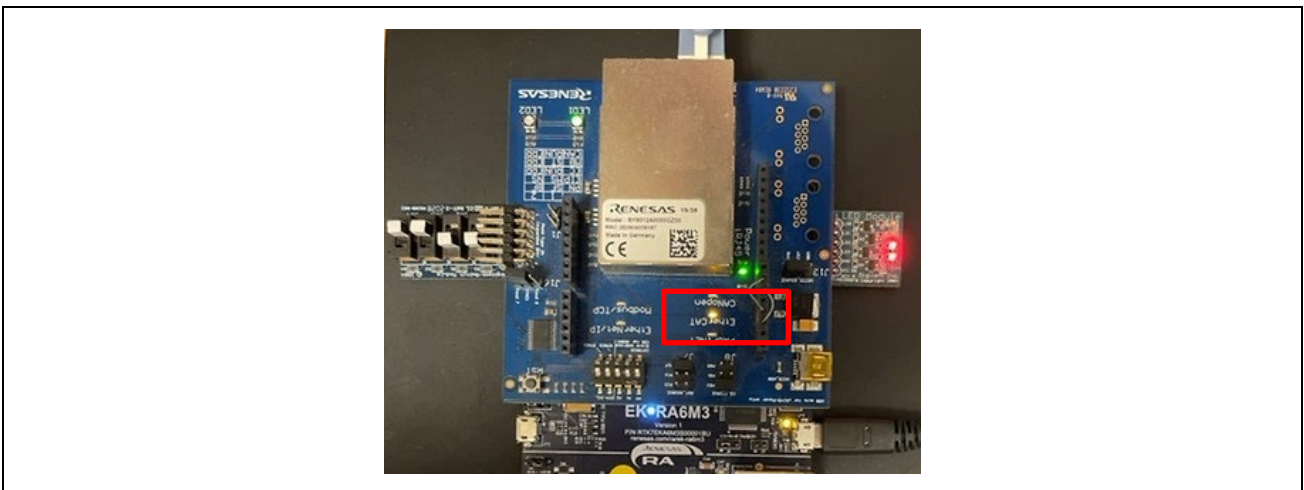
Figure 3-43 Protocol LED: EtherCAT
