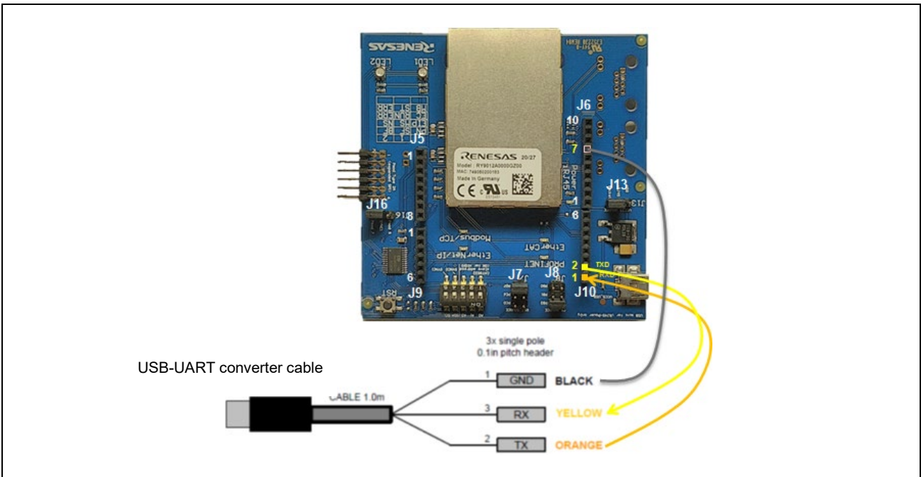
Figure 4-1 Connection of this board and USB-UART converter cable
