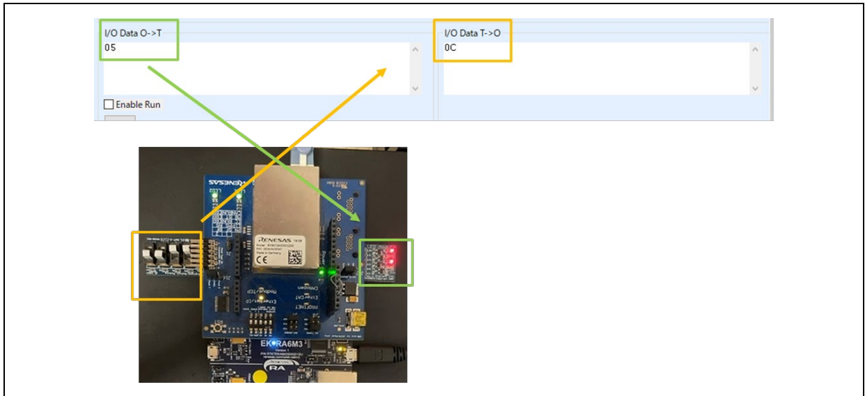
Figure 3-41 Remote-IO (LED/Switch) control [EtherNet/IP]
