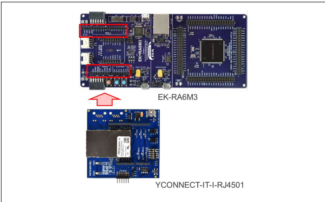
Figure 2-2 Arduino™ Connection
