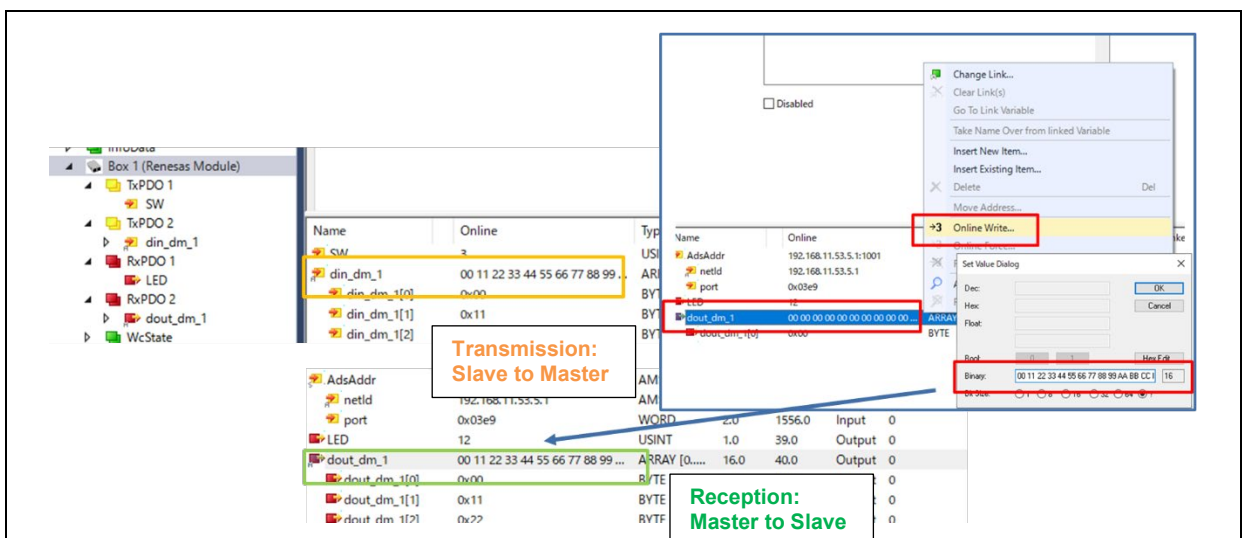
Figure 3-49 Mirror control [EtherCAT]
