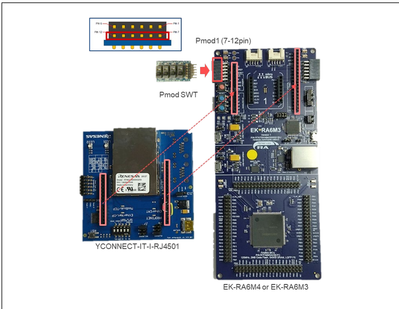
Figure 2-3 Multi-protocol Selector Connection
