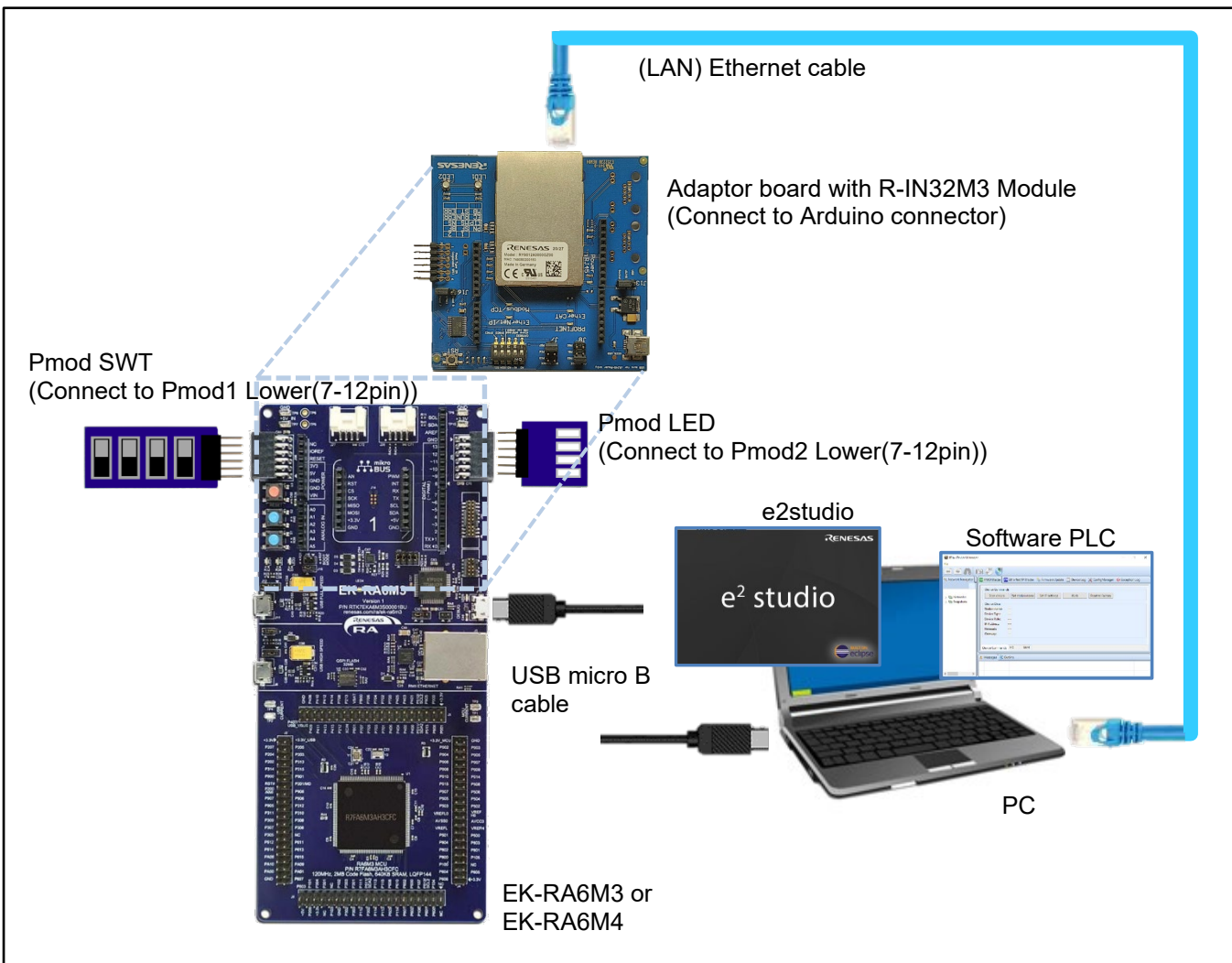
Figure 3-2 Connection configuration (connection with Pmod SWT and Pmod LED)
