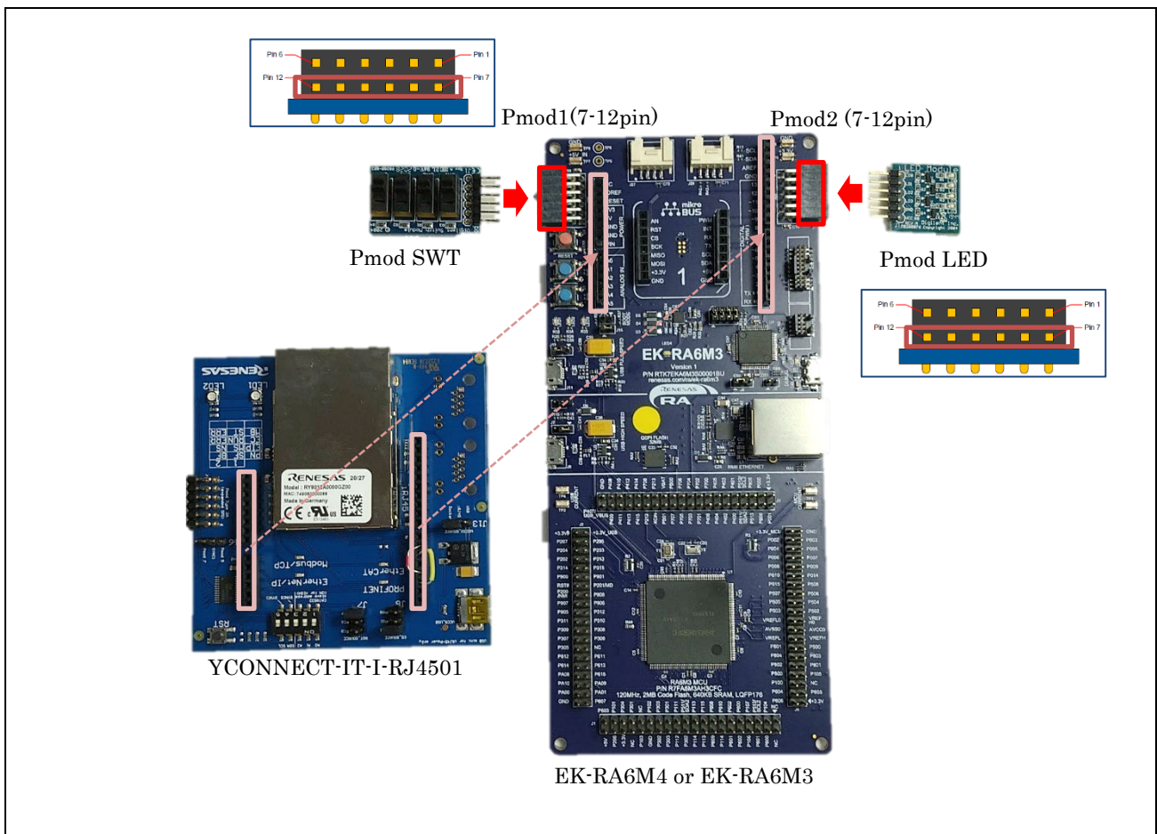
Figure 2-4 Remote I/O Connection
