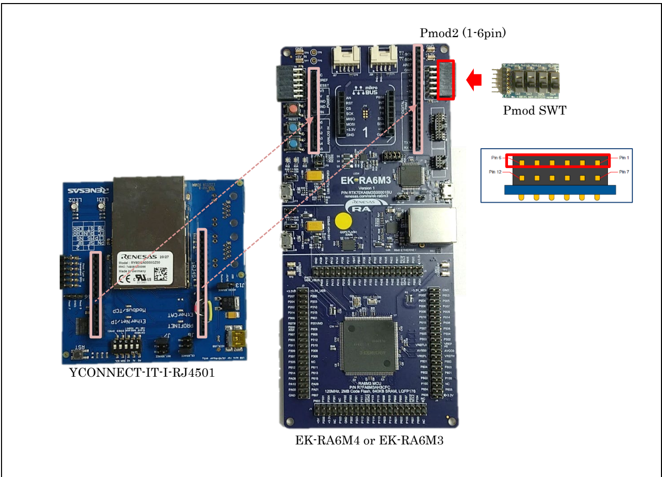
Figure 2-5 EtherCAT Explicit Device ID Connection
