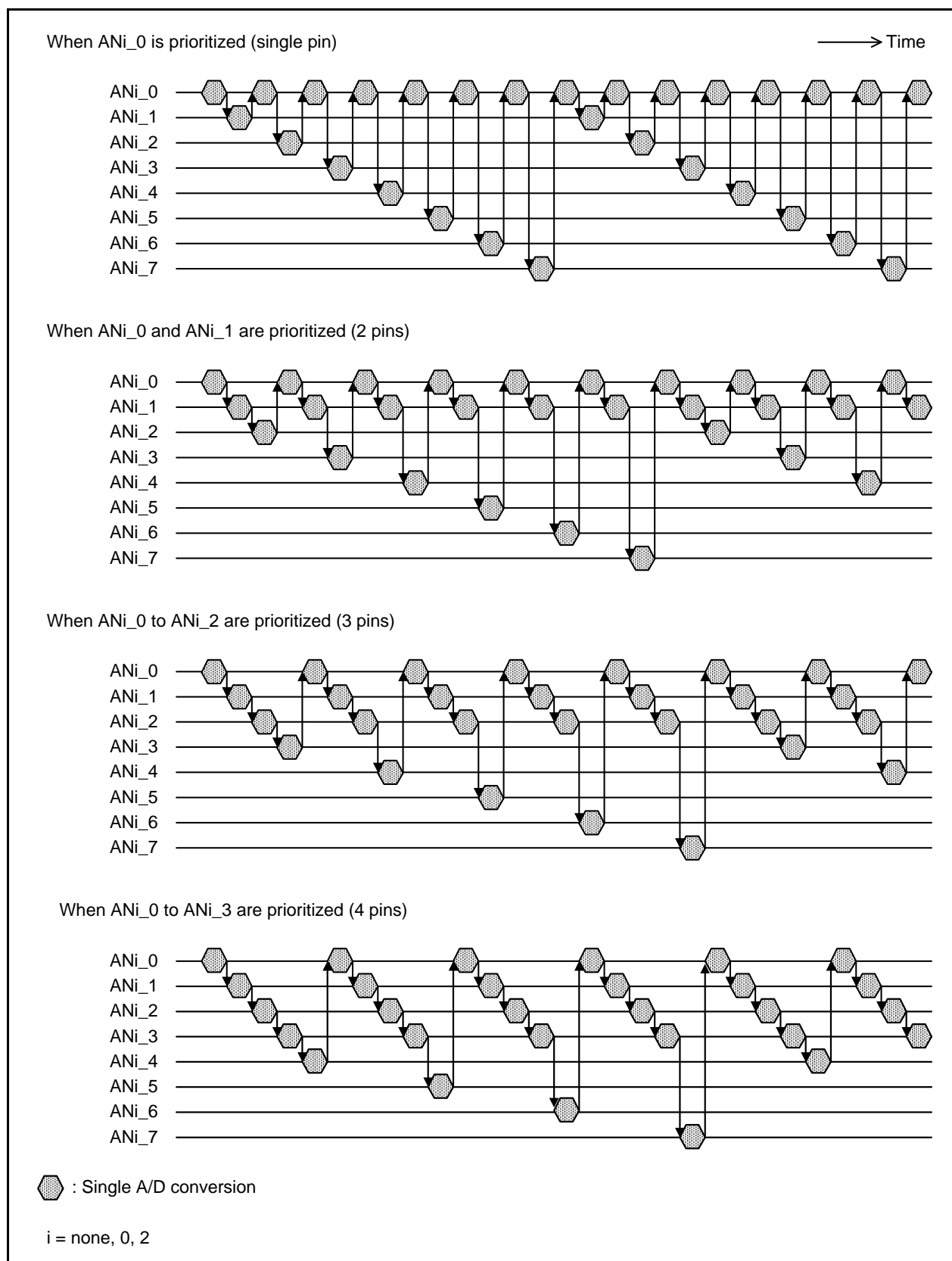
Figure 3.1 Transition Diagram of Pins Used During A/D Conversion in Repeat Sweep Mode 1
