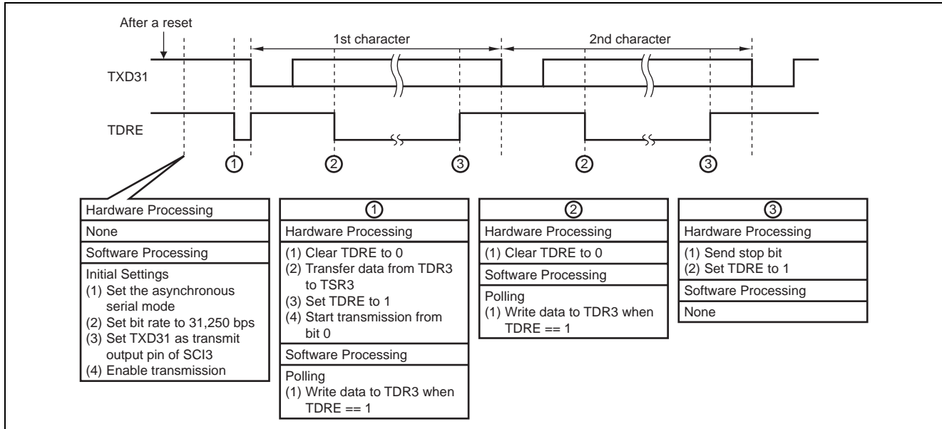
Figure 4 Principles of Operation for Serial Data Transmission in the Asynchronous Mode
