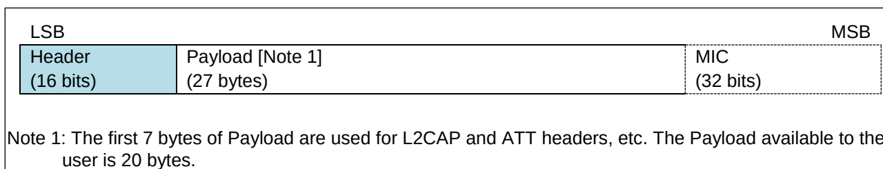
Figure 2-2 Data Channel PDU Structure (for Bluetooth Ver. 4.1)
