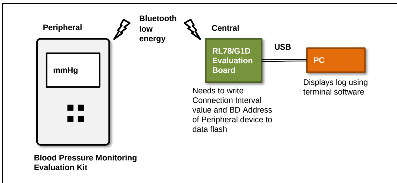
Figure 3-1 High-Speed Data Transfer Operation Demo System Configuration
