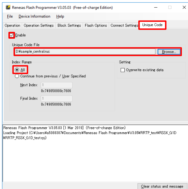
Figure 2-14 RFP "Unique Code" Tab
