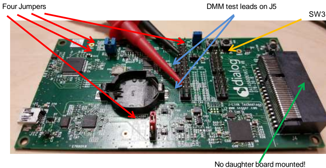
Figure 1: DA14580 PRO Kit Motherboard Connections for Calibration
