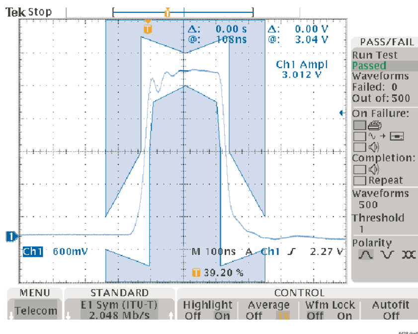
Figure 5b. E1 Pulse Mask - Primary Card Transmits, Secondary Card Powered Down
