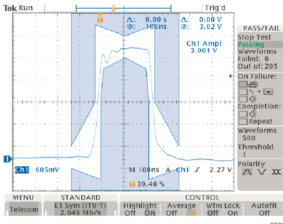
Figure 5a. E1 Pulse Mask - Primary Card Transmits, Secondary Card Standby
