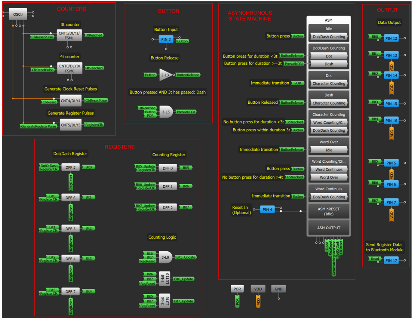
Figure 4. GreenPAK Designer overview highlighting the functional groups used in this project
