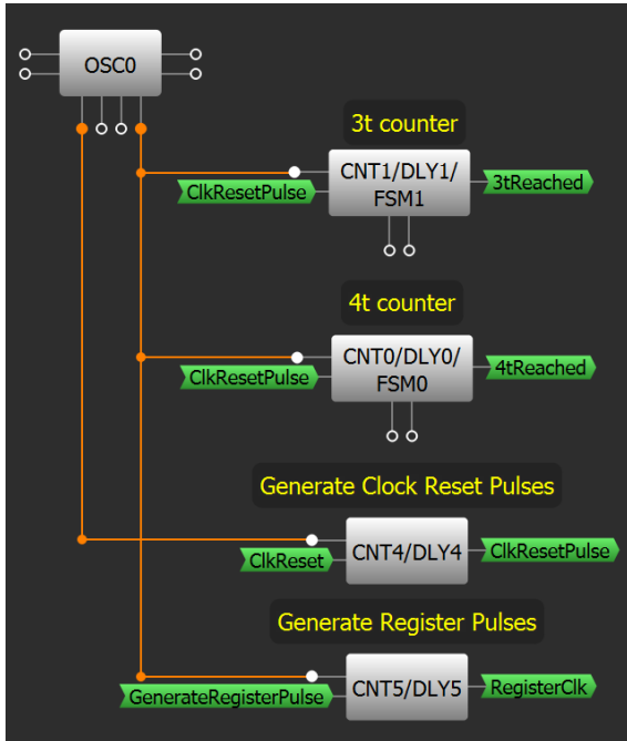
Figure 7. Four Counter blocks are used, two for timing and two for generating one-shot pulses
