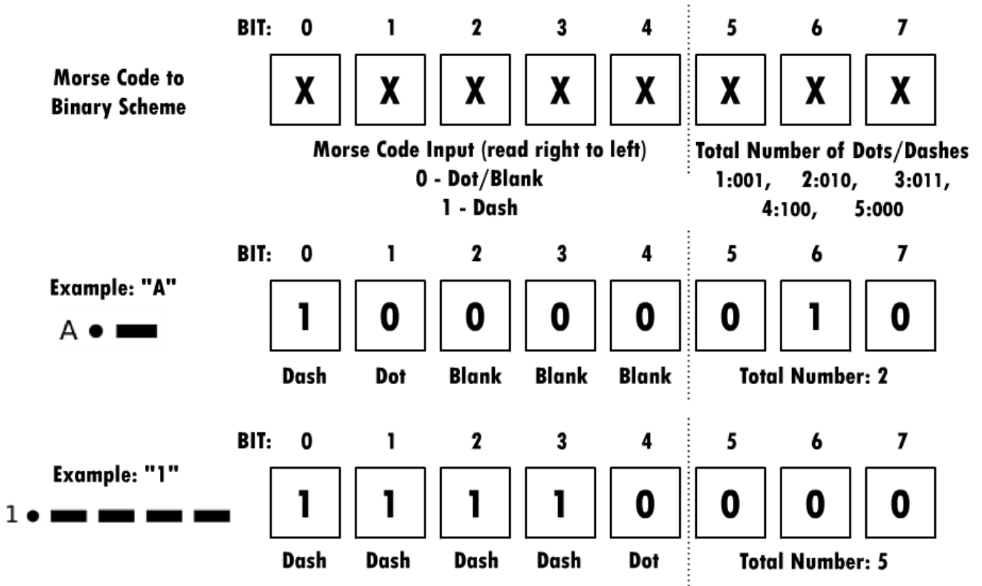
Figure 2. Conversion from Morse Code input to byte of alphanumeric data
