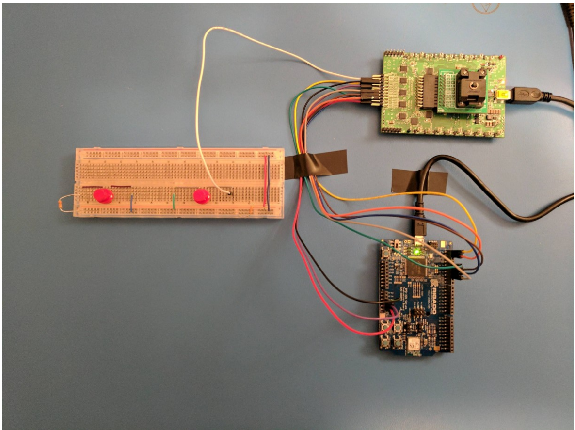
Figure 14. Picture of the wired connections between the breadboard input button, the GreenPAK Development Board (green), and the Bluetooth module's evaluation board (blue). The left button on the breadboard functions as the ASM reset and has been disconnected.
