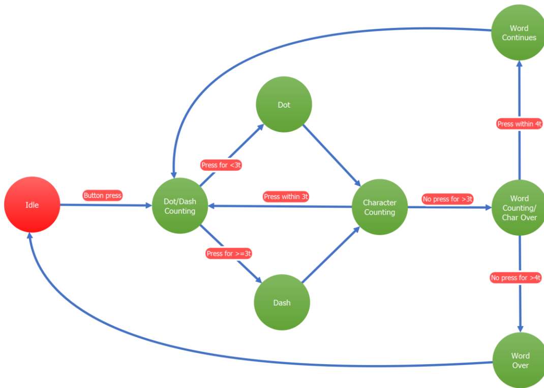
Figure 3. State diagram of Morse Code input conversion. The variable t represents one unit of Morse Code time (see Morse Code reference in Figure 1). Some alterations have been made with regards to timing to simplify the Morse Code input
