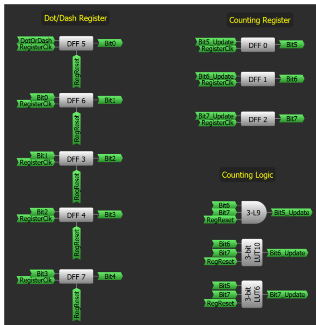
Figure 10. One register is used to record the user input, and the other is used to keep track of the total number of dots and dashes
