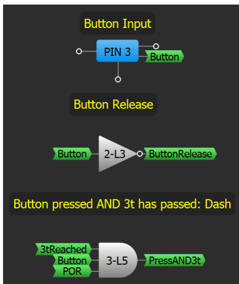
Figure 12. PIN 3 records the Morse Code input, and two LUTs pass additional information to the ASM
