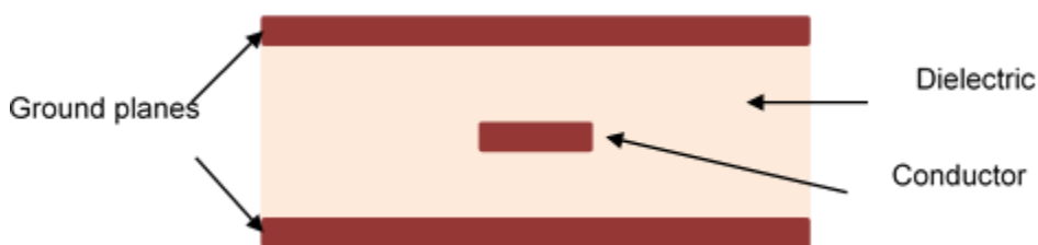
Figure 2. Stripline
