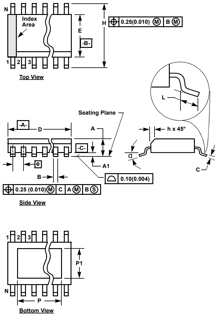
M8.15C 8 Lead Narrow Body Small Outline Exposed Pad Plastic Package (EPSONC)
