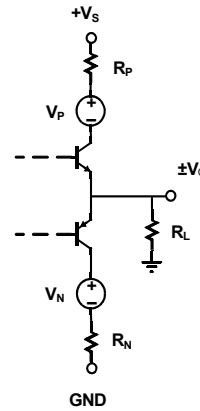
FIGURE 51. HEADROOM MODEL
