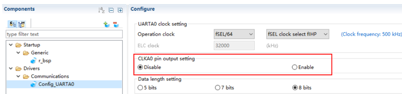
Figure 3-4 CLKA0 pin output selection
