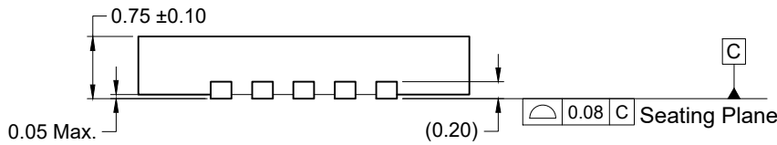
SIDE VIEW
