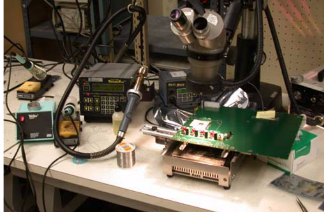
Figure 6. Hot Plate Rework Station Overview
