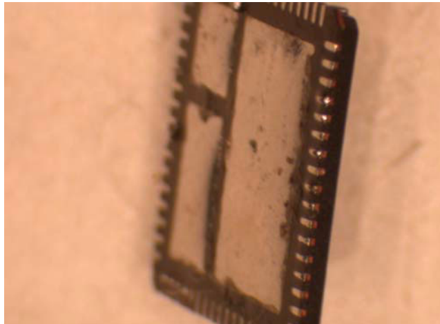
Figure 16. Finished Tinned Thermal Land on QFN
