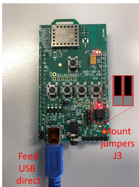
Figure 1 Connection setup for reprogramming
