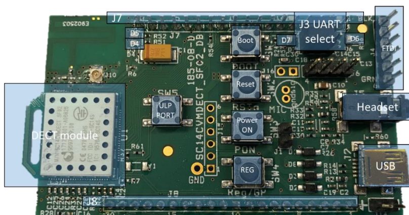
Figure 2 Overview of the SC14CVMDECT_SF01
