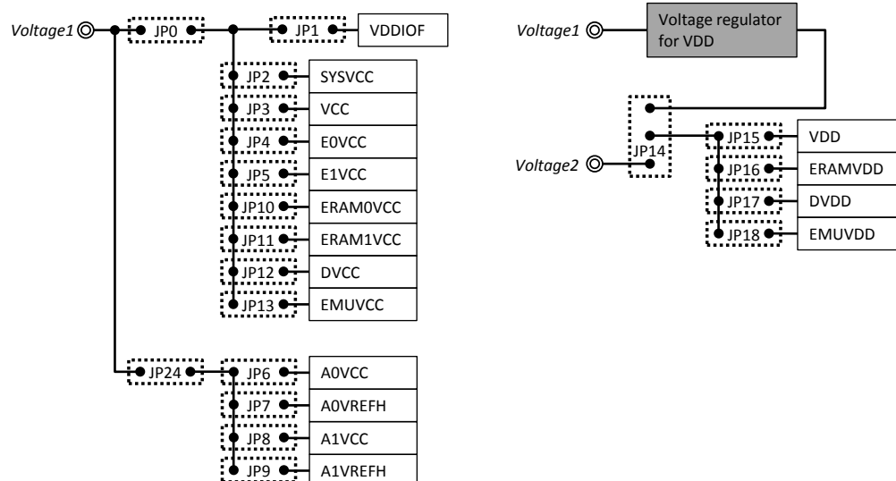
Figure 4 Voltage Distribution on the PiggyBack Board
