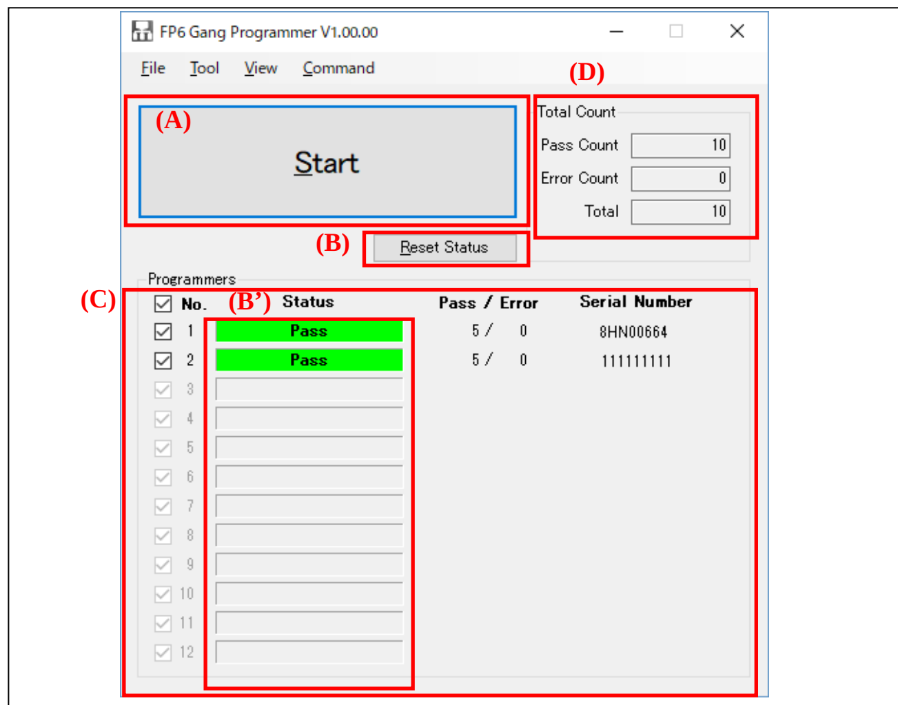
Figure 5 Main Window
