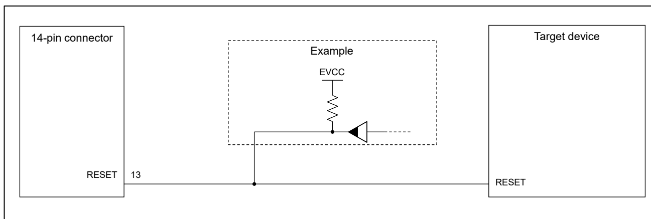
Figure 2-9 Example of Connecting a Reset Circuit
