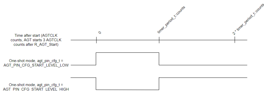
Figure 144: AGT One-Shot Output
