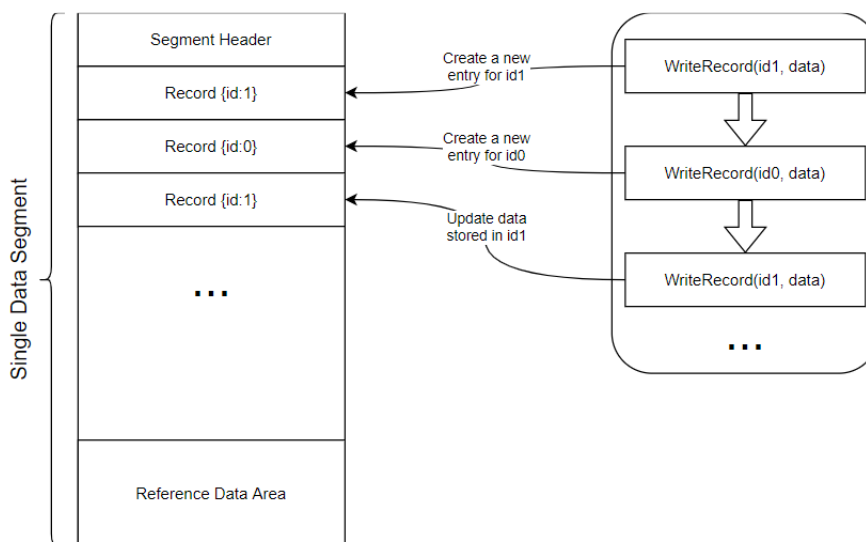
Figure 231: Segment Data Format
