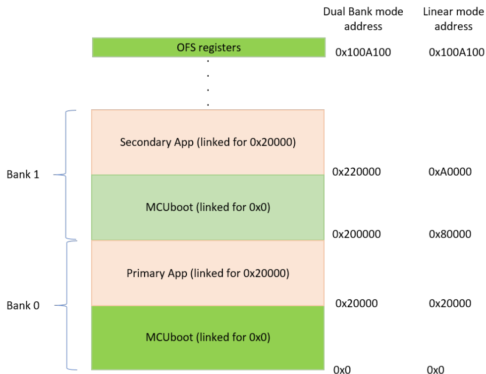
Figure 207: MCUboot Dual Bank layout for 1 MB Memory
