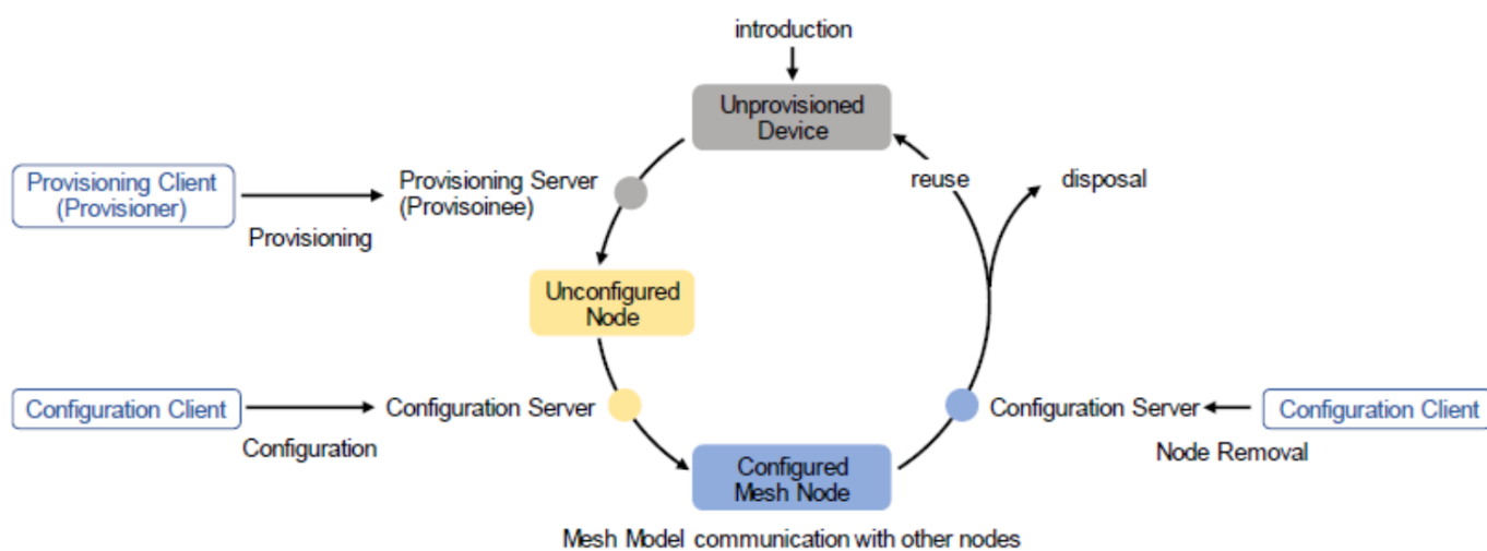
Figure 141: Device Life Cycle Image
