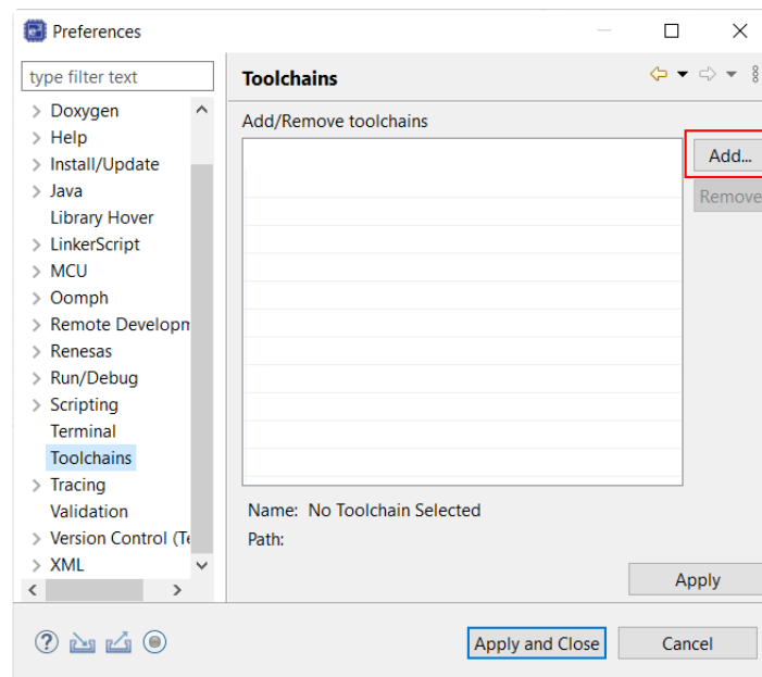
Figure 53: Add Toolchain
