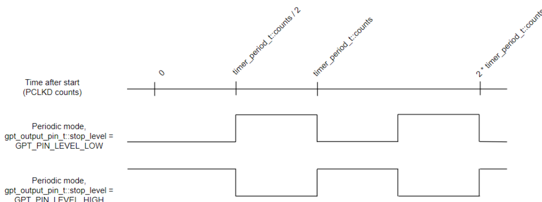
Figure 168: GPT Periodic Output
