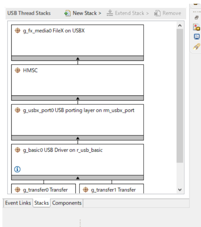
Figure 223: FileX on USBX Stack
