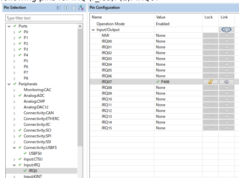
Figure 228: IRQ Pin Setting
