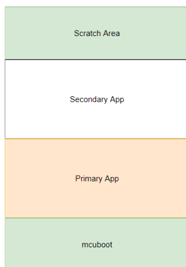
Figure 208: MCUboot Memory Map
