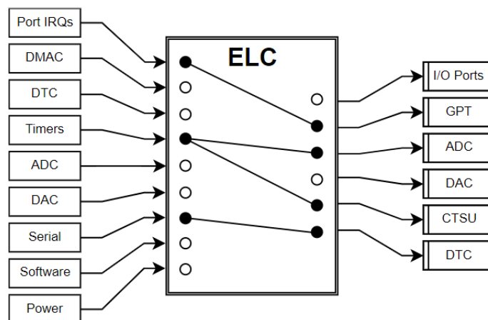
Figure 161: Event Link Controller Conceptual Diagram
