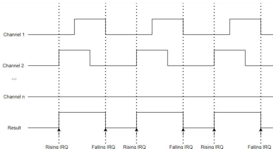
Figure 175: IPLS IRQ Generation
