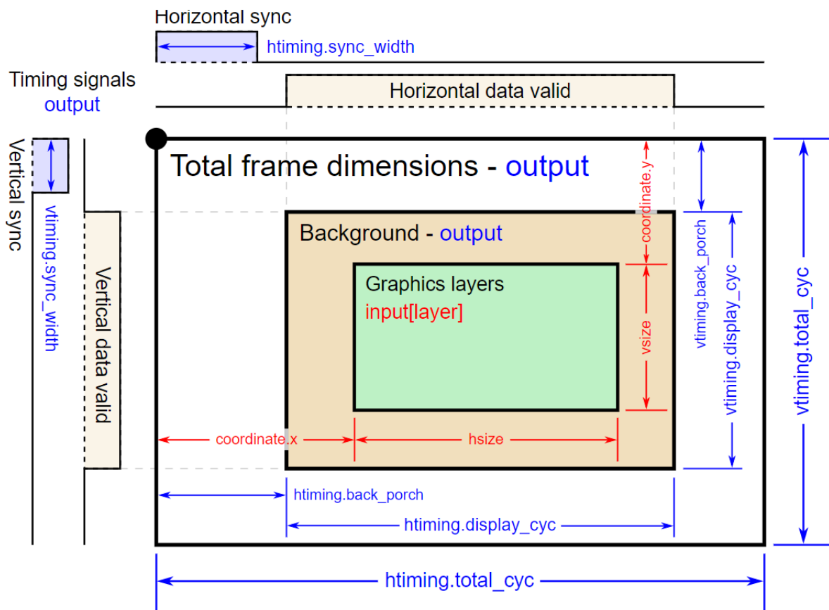
Figure 166: GLCDC layers and timing
