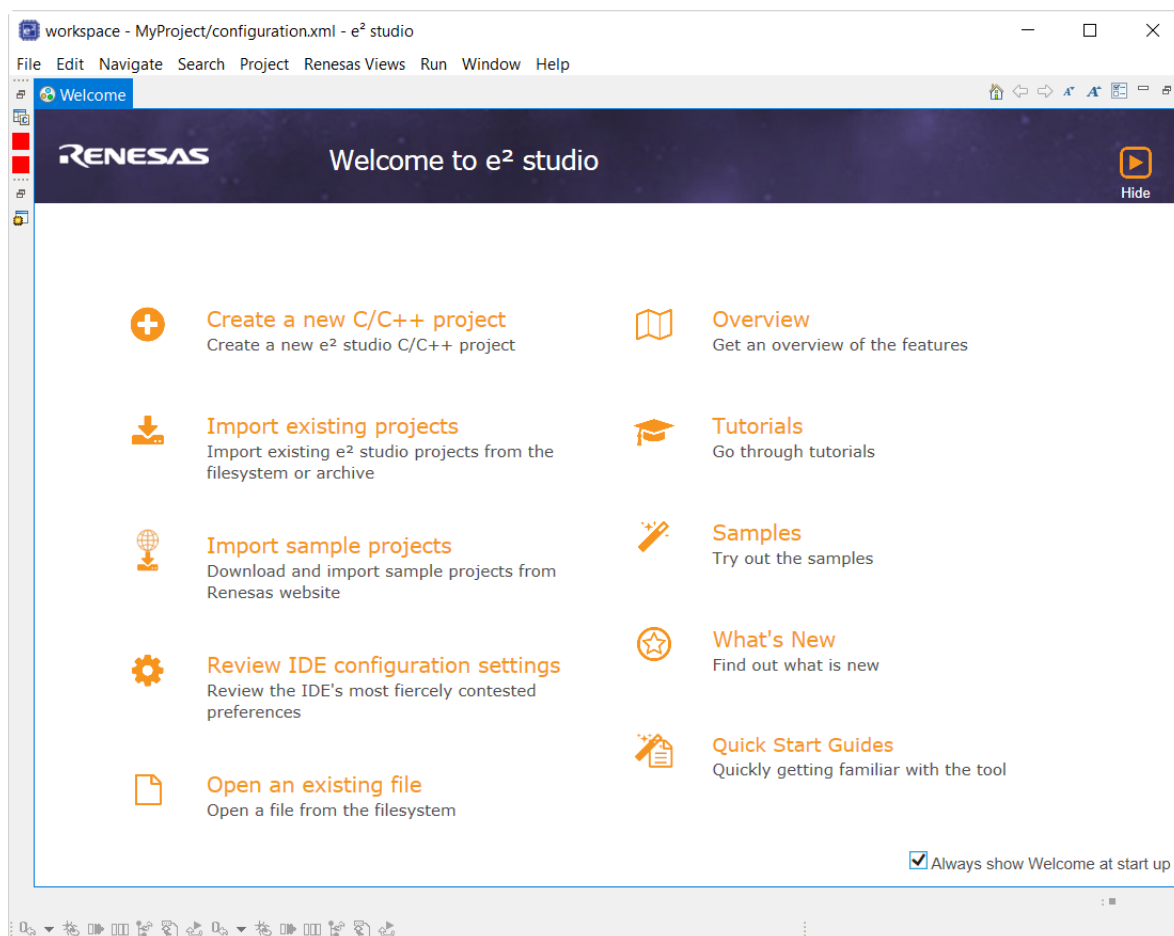
Figure 37: Welcome window
