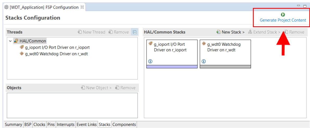
Figure 93: Generate Project Content button
