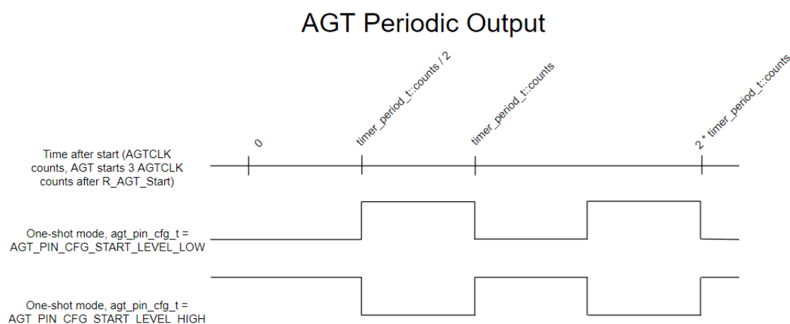
Figure 145: AGT Periodic Output
