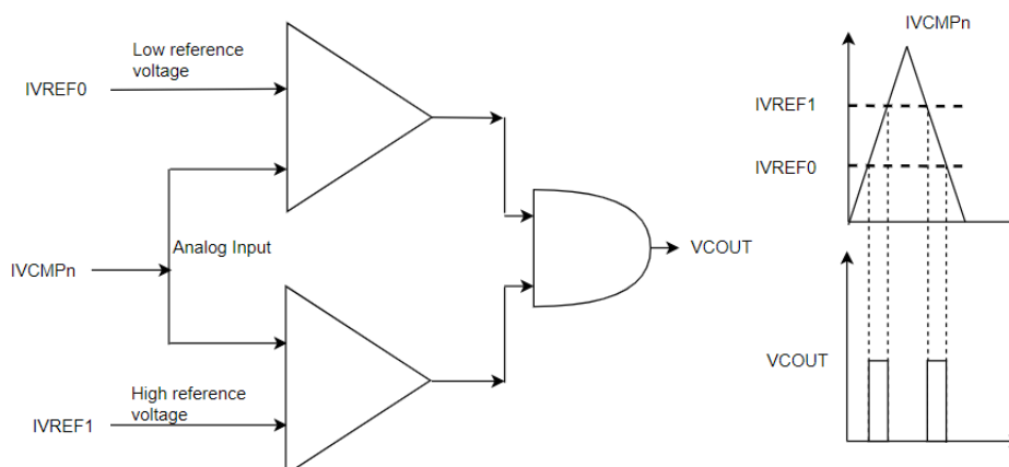
Figure 143: ACMLP Window Mode Operation
