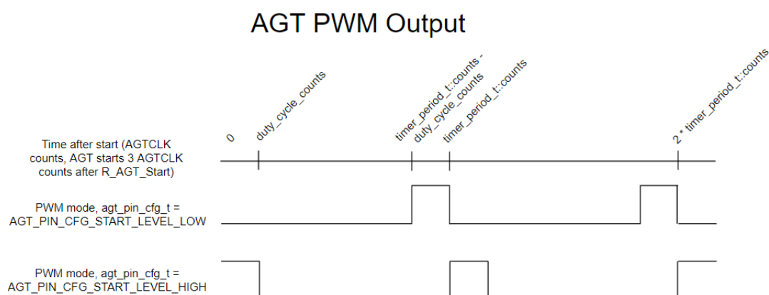
Figure 146: AGT PWM Output
