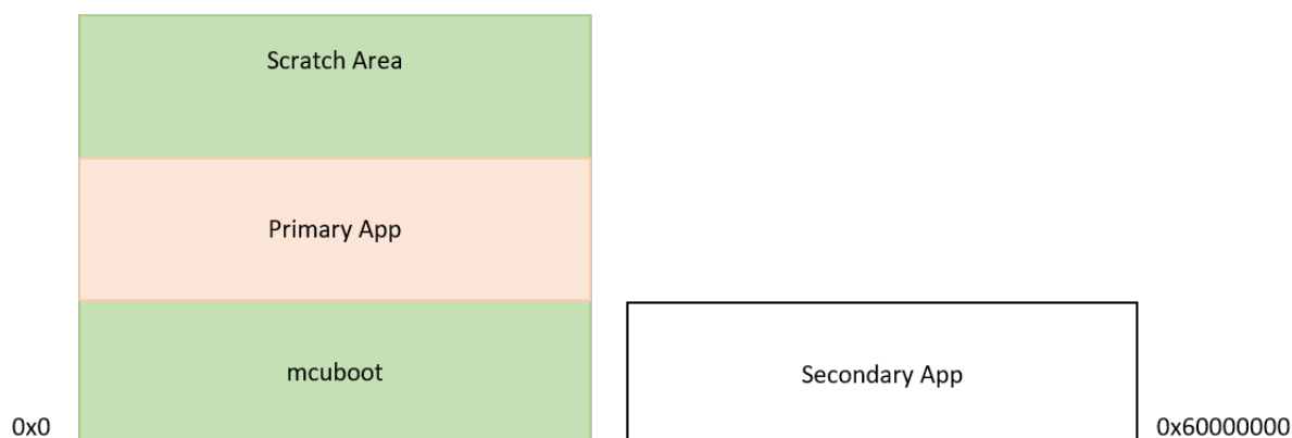
Figure 210: MCUboot Memory Map with QSPI
