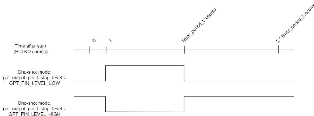
Figure 167: GPT One-Shot Output
