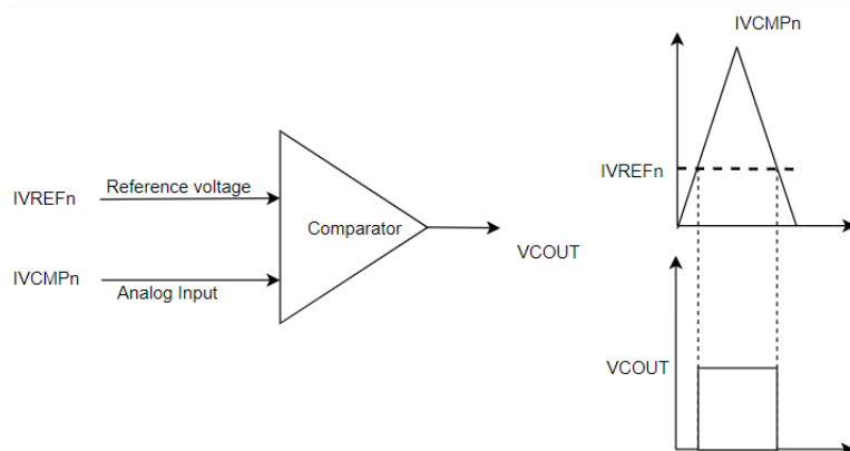
Figure 142: ACMLP Standard Mode Operation
