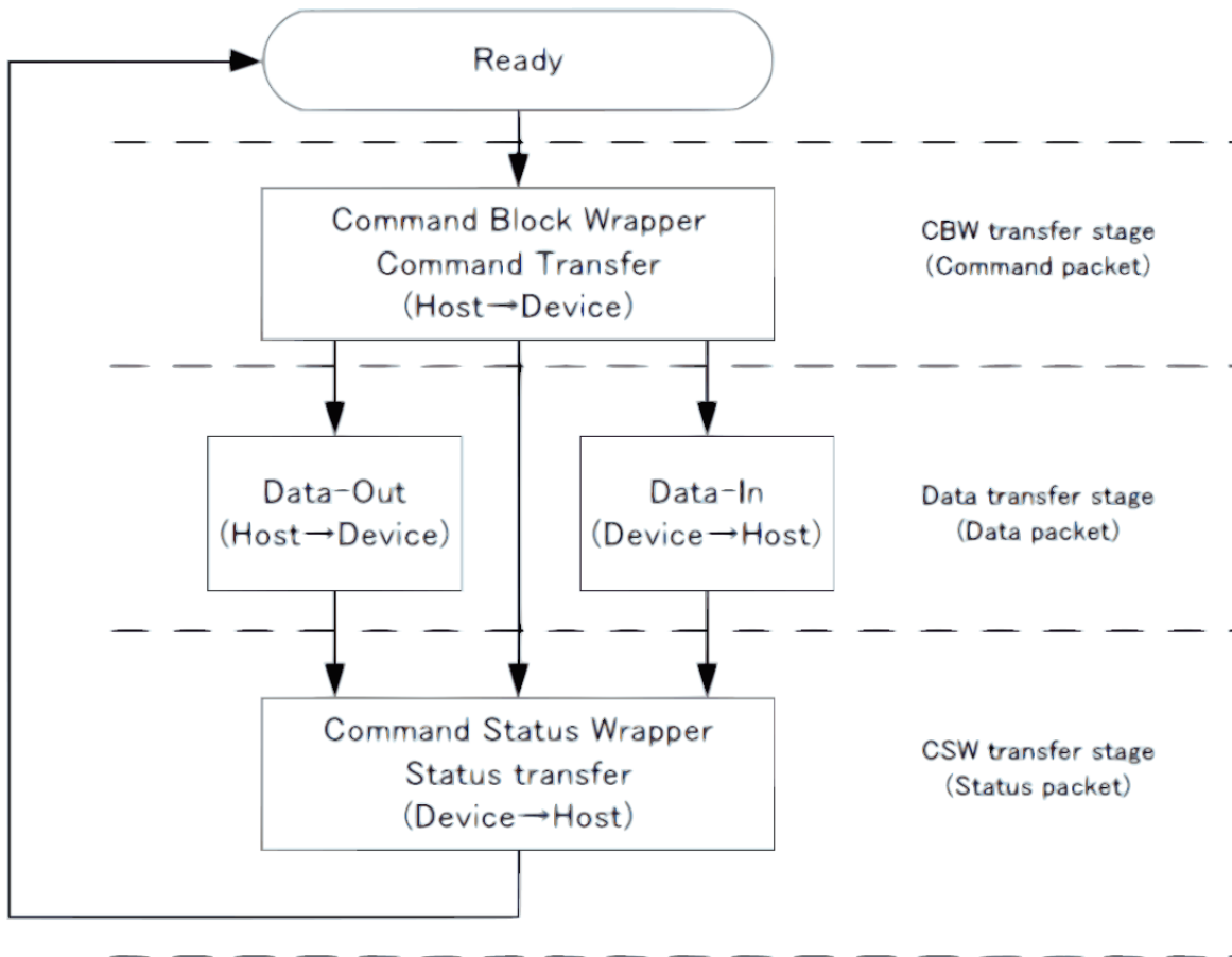
Figure 200: BOT protocol Overview
