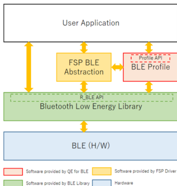
Figure 148: BLE software structure
