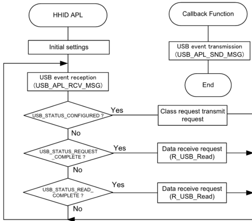
Figure 188: Main Loop (Normal mode)
