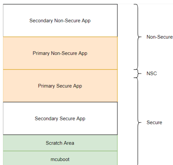
Figure 209: MCUboot Memory Map (TrustZone)
