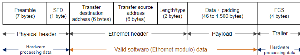
Figure 163: Frame Format Image
