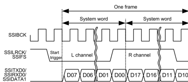
Figure 176: SSI Frame Diagram (8-bit word, 8-bit samples)
