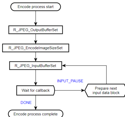
Figure 174: JPEG Encode Operational Flow
