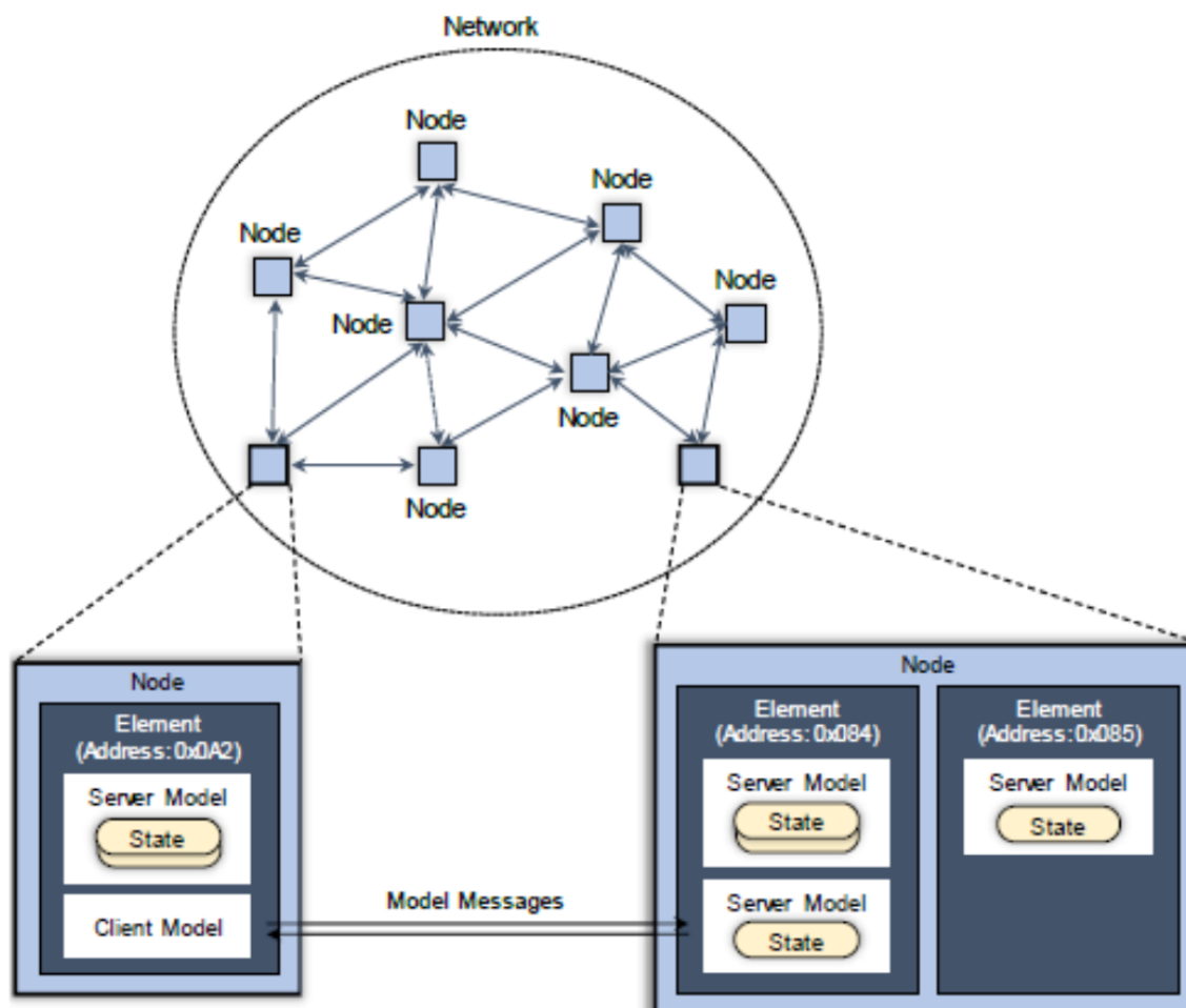
Figure 140: Overview Of Bluetooth Mesh
