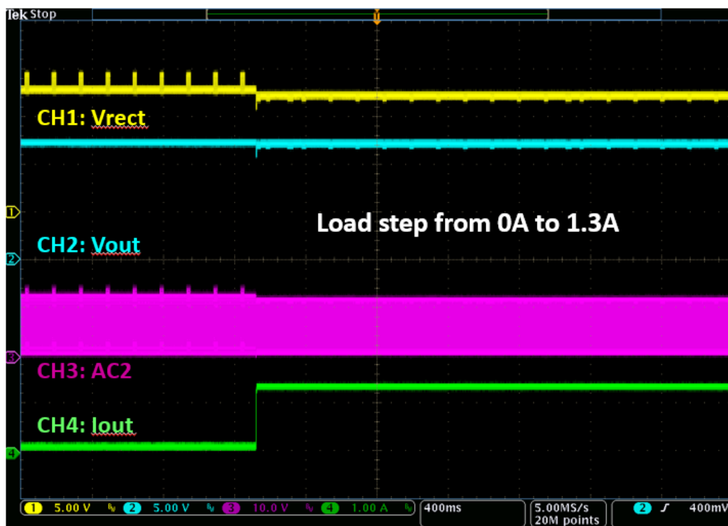
Figure 10. Load Transient Response (Iout Change from 0A to 1.3A)
