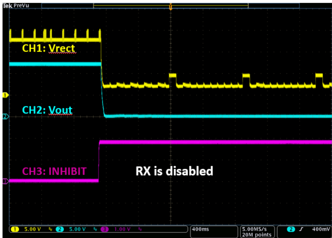
Figure 11. INHIBIT Operation
