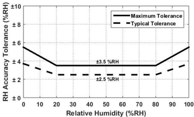
Figure 6. HS3103 RH Accuracy Tolerance at 25°C
