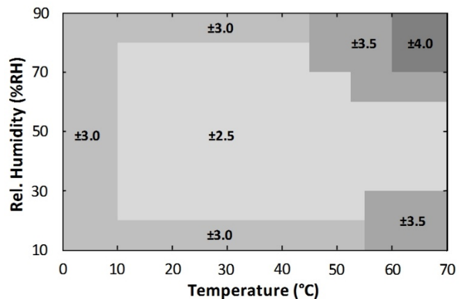
Figure 7. HS3103 RH Accuracy over Temperature
