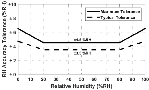
Figure 8. HS3104 RH Accuracy Tolerance at 25°C
