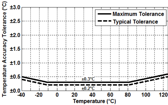
Figure 10. HS3101/HS3102 Temperature Sensor Accuracy Tolerance
