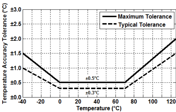
Figure 12. HS3104 Temperature Sensor Accuracy Tolerance
