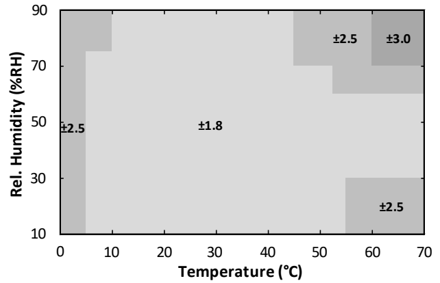
Figure 5. HS3102 RH Accuracy over Temperature
