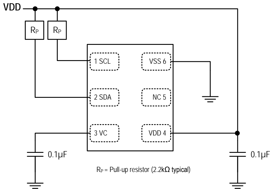
Figure 17. HS310x Application Circuit (Top View)
