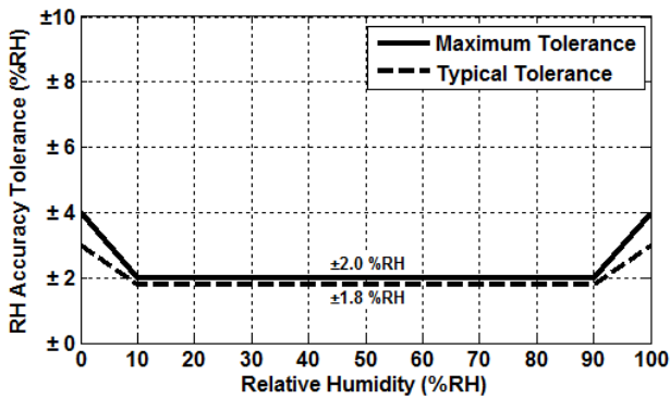
Figure 4. HS3102 RH Accuracy Tolerance at 25°C
