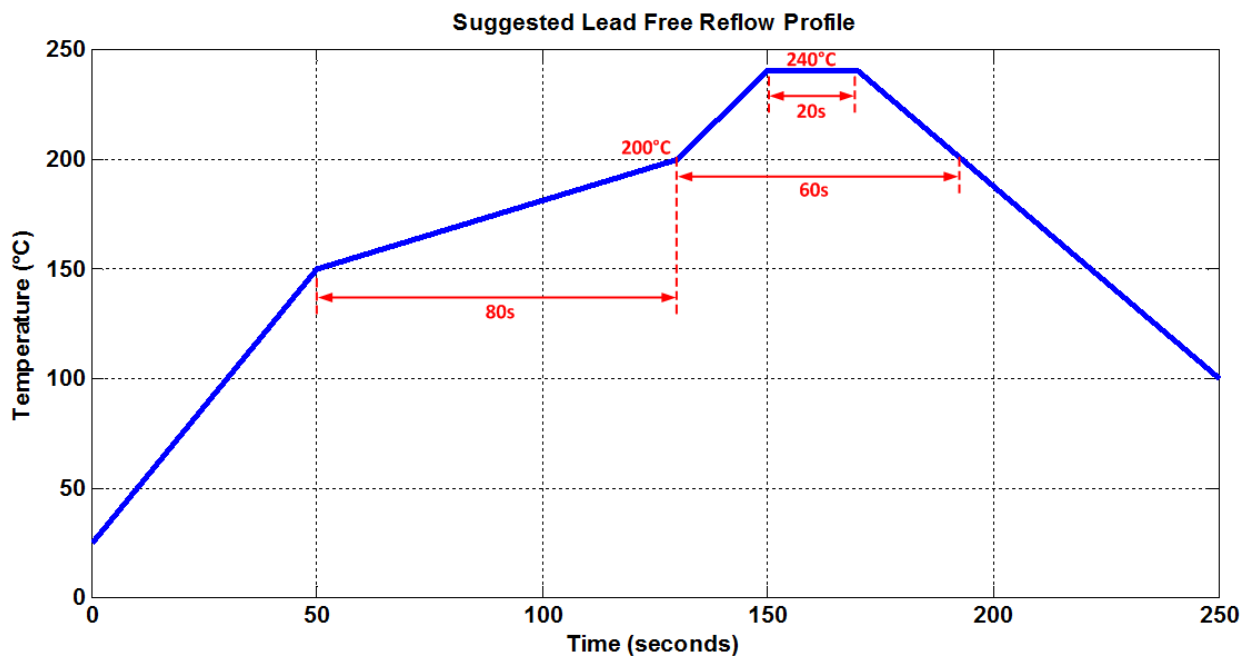
Figure 19. Recommended Soldering Profile
