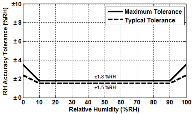
Figure 2. HS3101 RH Accuracy Tolerance at 25°C
