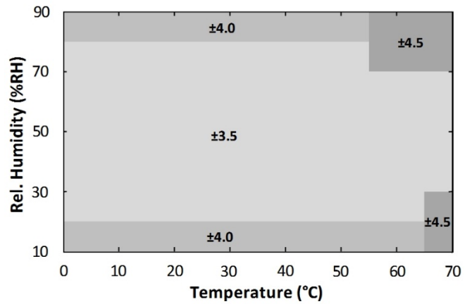
Figure 9. HS3104 RH Accuracy over Temperature
