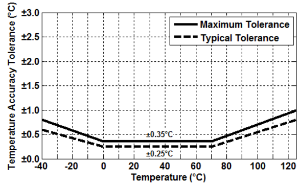
Figure 11. HS3103 Temperature Sensor Accuracy Tolerance
