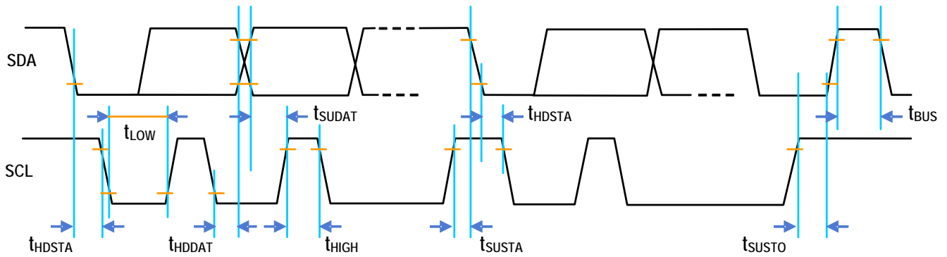
Figure 13. Timing Diagram
