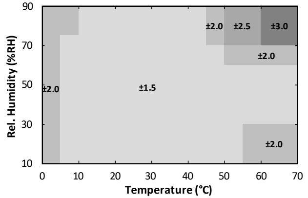
Figure 3. HS3101 RH Accuracy over Temperature
