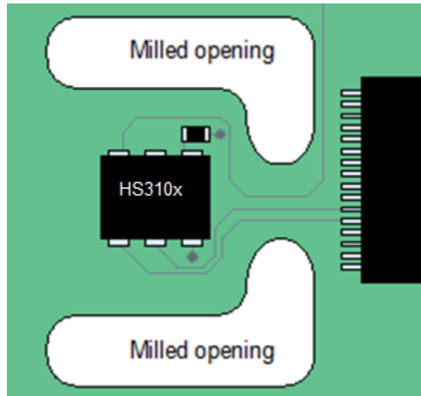
Figure 20. Milled PCB Openings for Thermal Isolation
