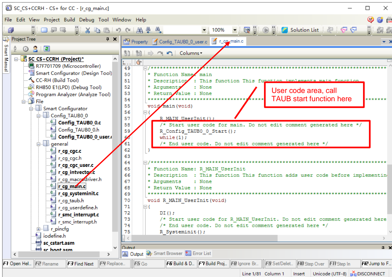
Figure 5-8. Add user code to main function
