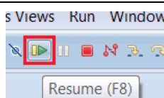
Figure 4. Resume button
